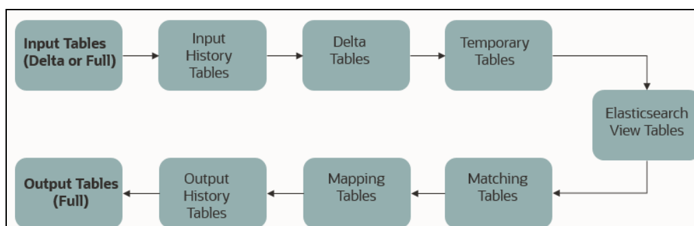
Figure 19: Entity Resolution
