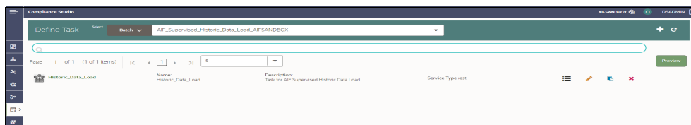
Figure 149: Define Task
