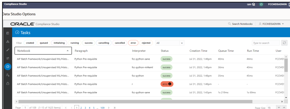
Figure 126: Tasks
