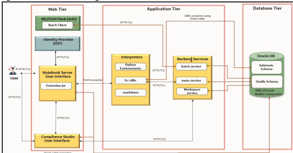
Figure 6: Scenario Authoring
