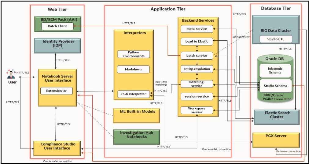
Figure 9: Investigation Hub
