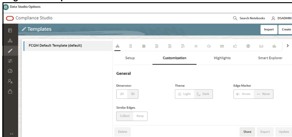
Figure 22: Template screens
