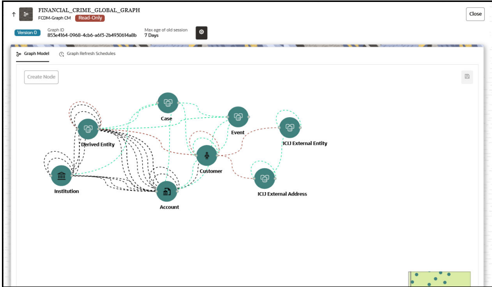
Figure 18: Graph Model
