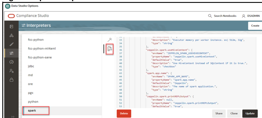
Figure 4: Spark Interpreter
