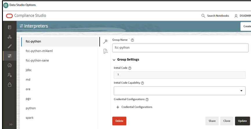
Figure 25: Interpreters
