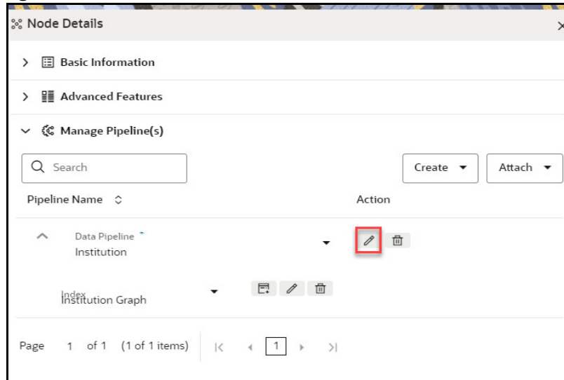
Figure 19: Node Details
