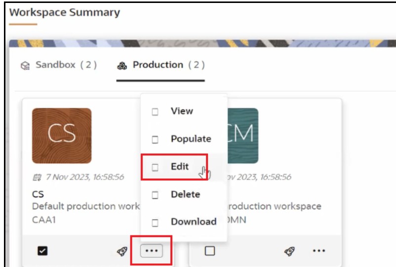
Figure 12: CS Workspace
