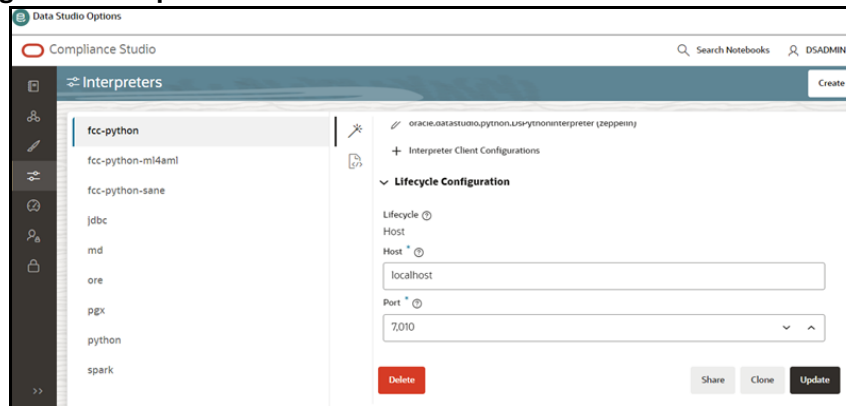
Figure 25: Interpreters
