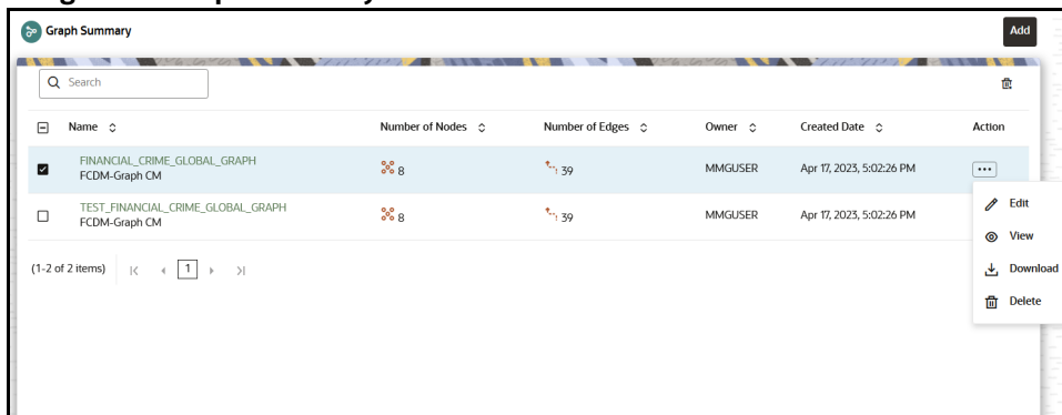
Figure 17: Graph Summary
