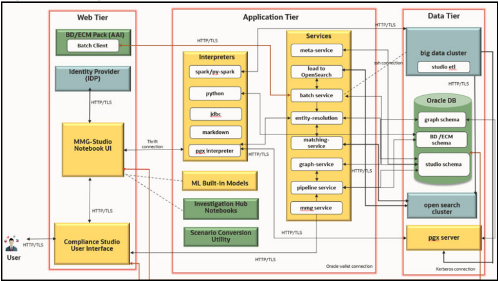
Figure 8: Investigation Hub
