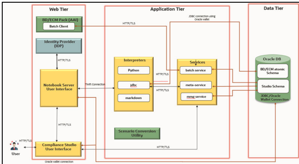
Figure 5: Scenario Authoring
