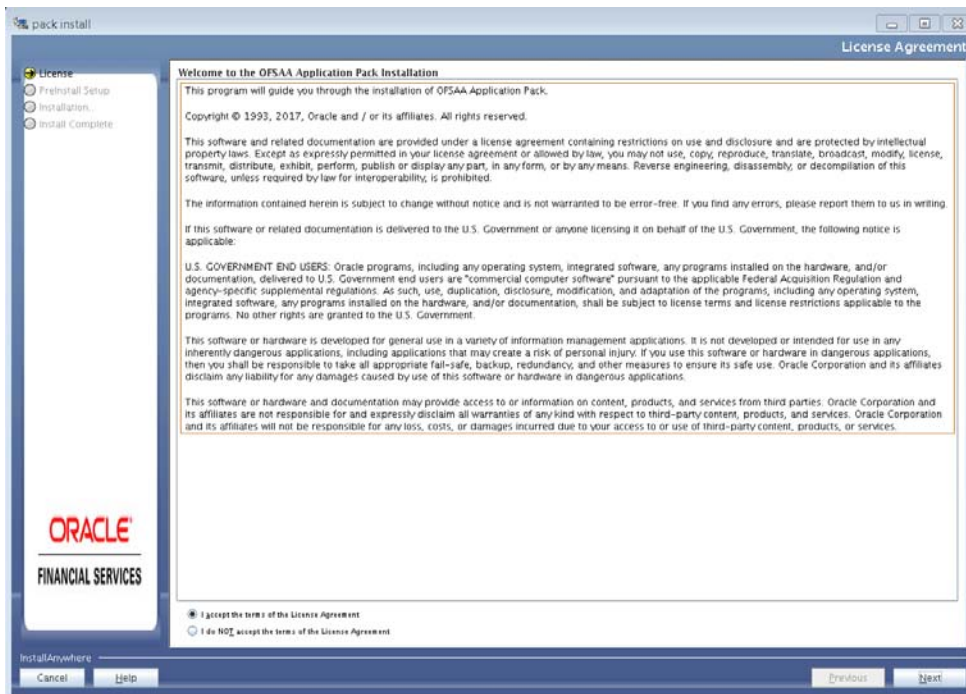
Figure 4–10 License Agreement
