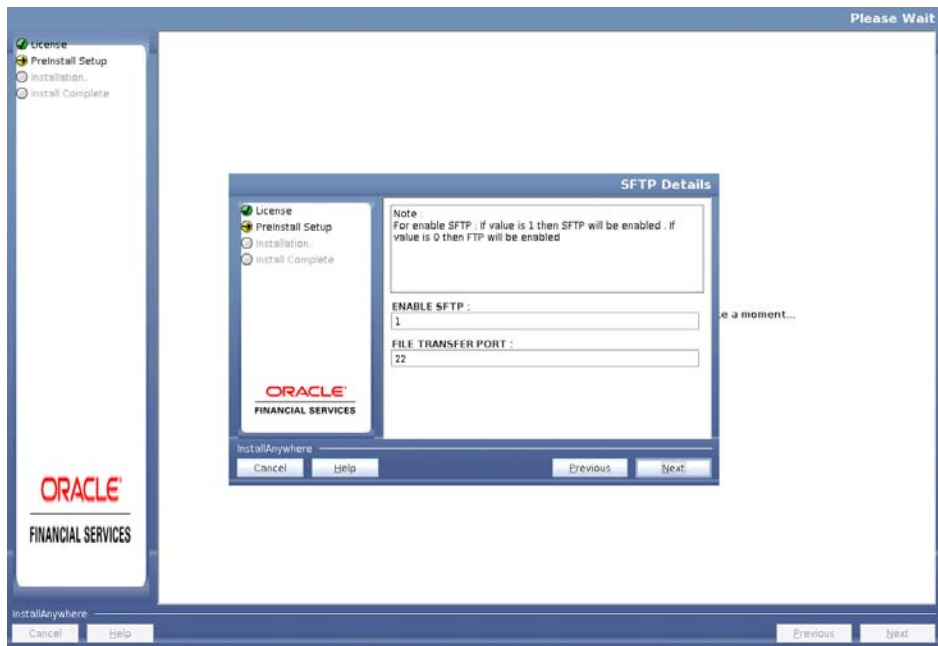
Figure 4–26 SFTP Details
