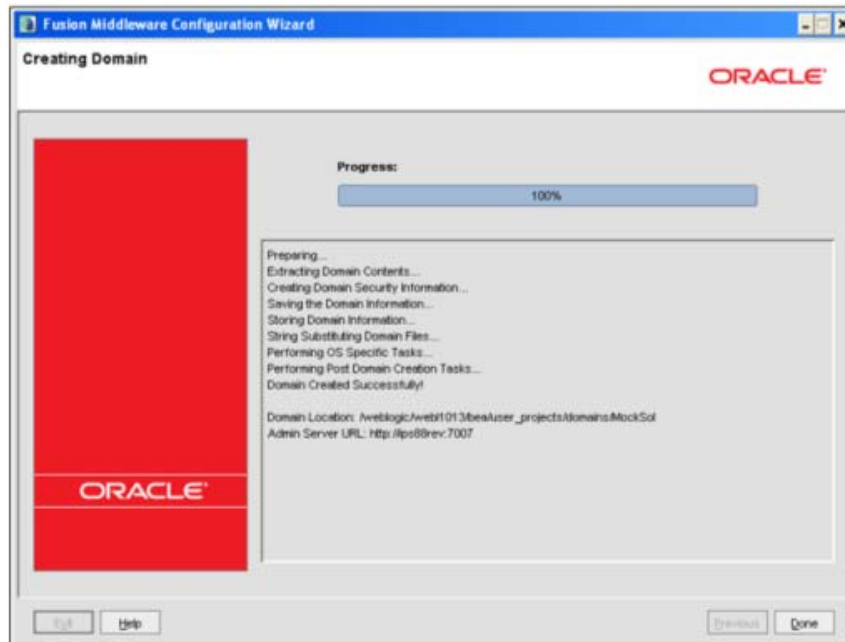
Figure 6–8 Creating Domain
