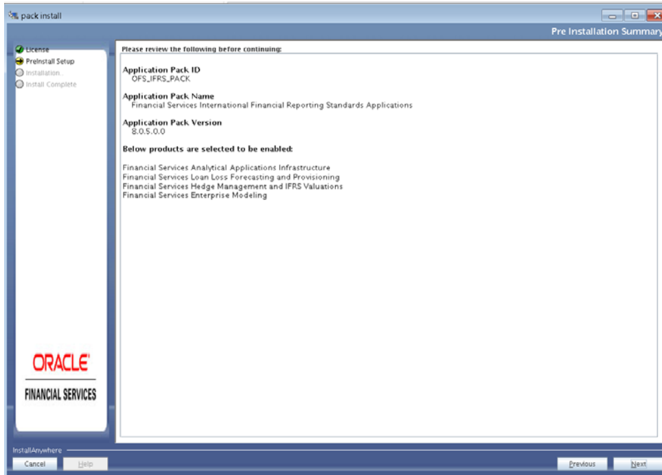
Figure 4–13 Pre-Installation Summary
