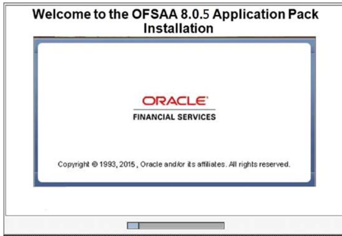
Figure 4–9 Initialization Window
