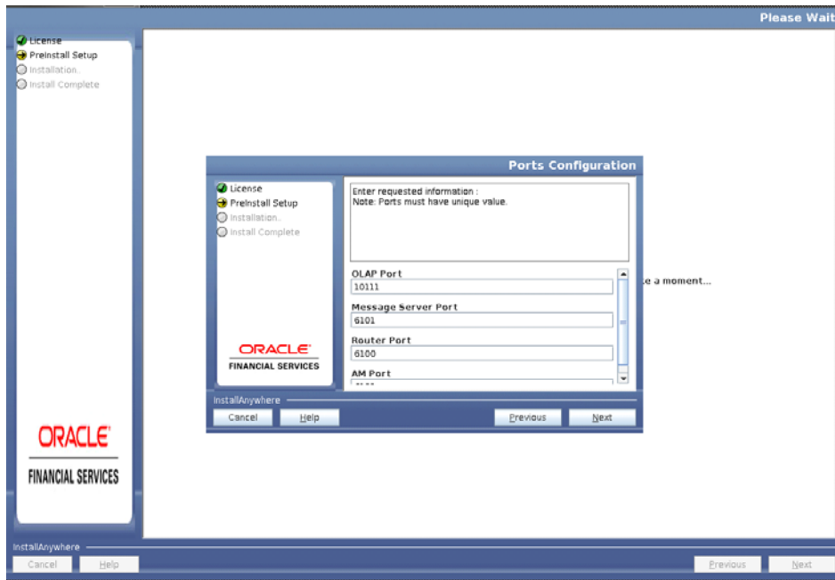
Figure 4–25 Ports Configuration
