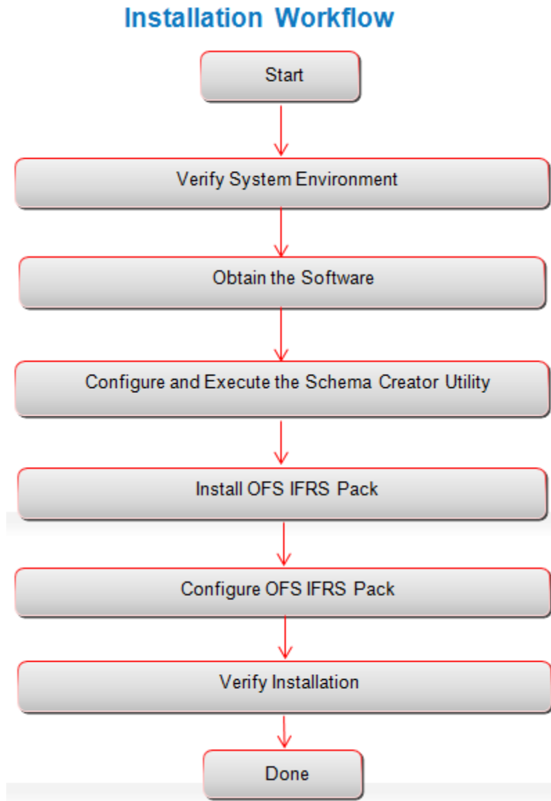
Figure 2–1 Installation Overview
