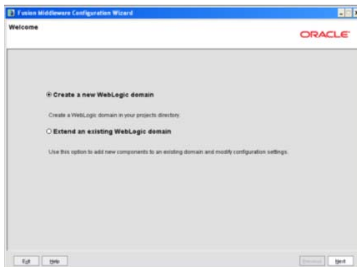
Figure 6–3 Welcome
