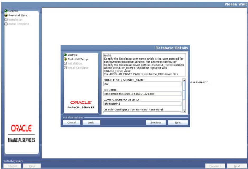
Figure 4–23 Database Details
