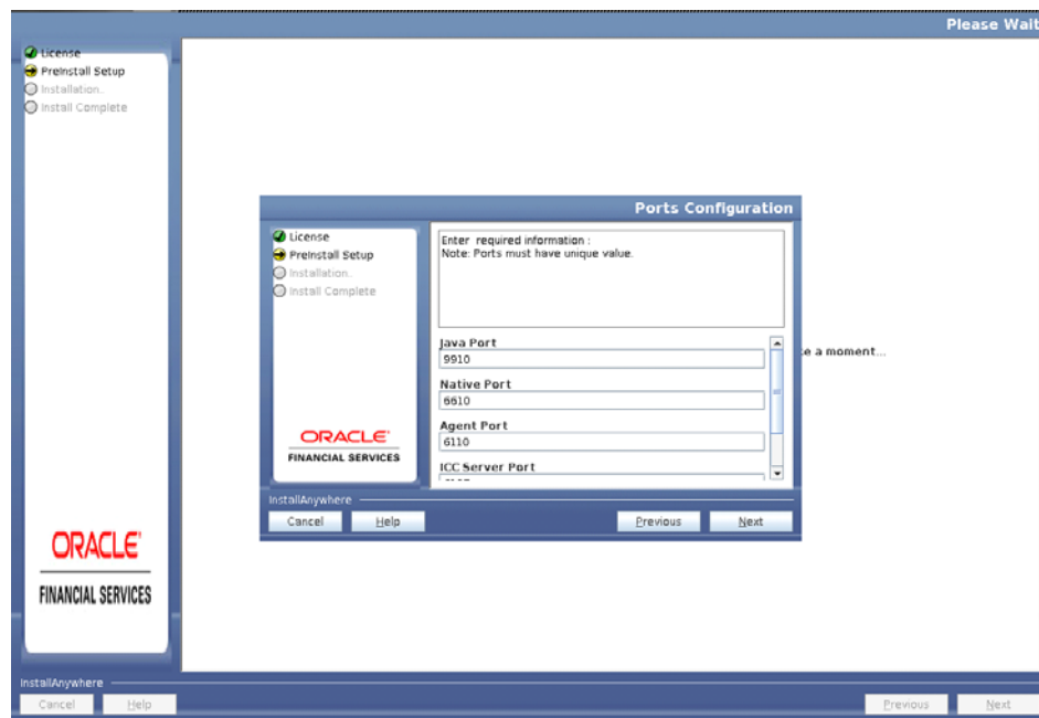
Figure 4–24 Ports Configuration
