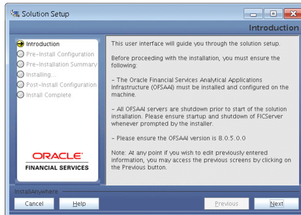
Figure 4–34 Installation Introduction
