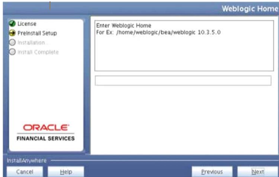
Figure 4–20 WebLogic Home
