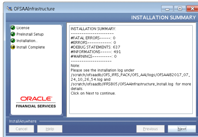
Figure 4–30 INSTALLATION SUMMARY
