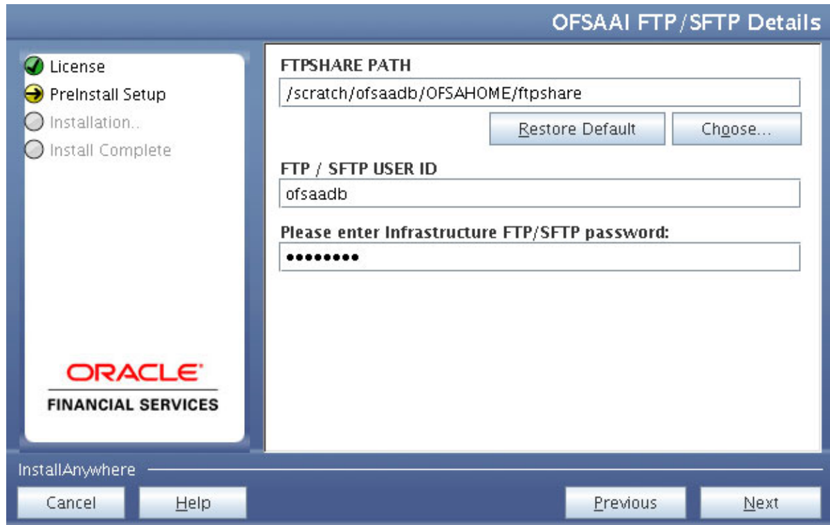
Figure 4–27 OFSAAI FTP/SFTP Details
