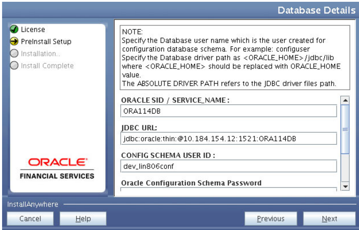
Figure 4–23 Database Details
