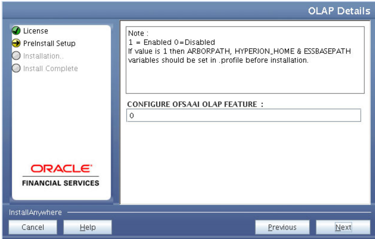
Figure 4–21 OLAP Details
