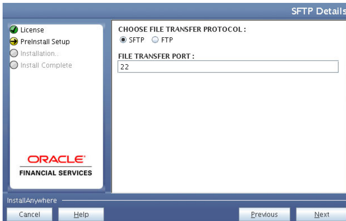
Figure 4–26 SFTP Details
