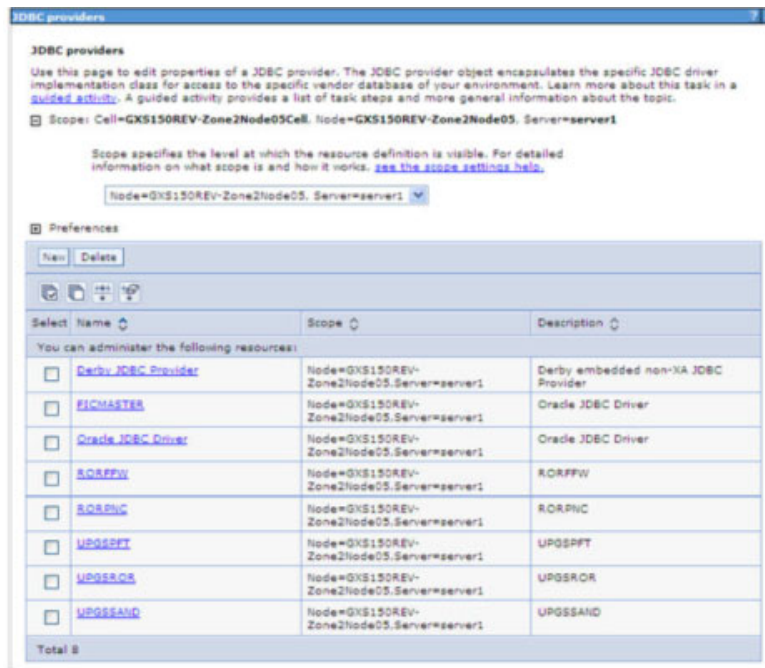
Figure 6–3 JDBC Providers
