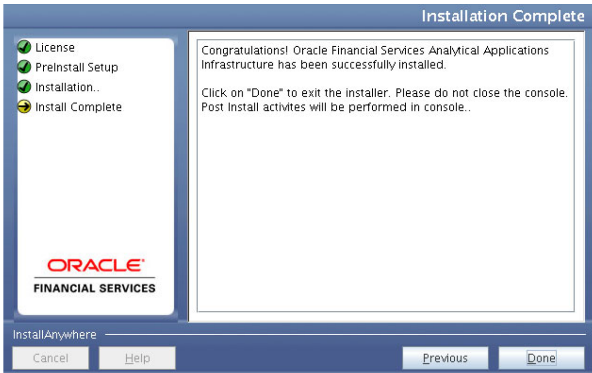
Figure 4–31 Installation Complete
