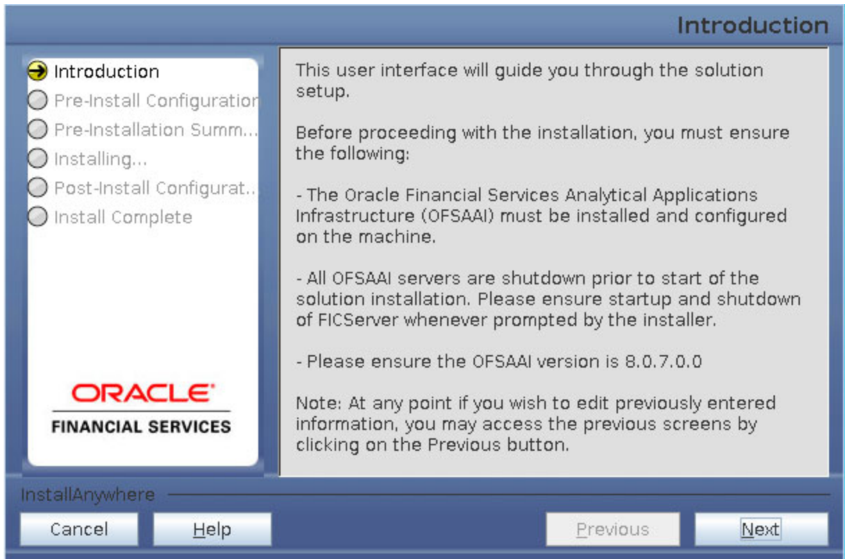
Figure 4-34 Installation Introduction
