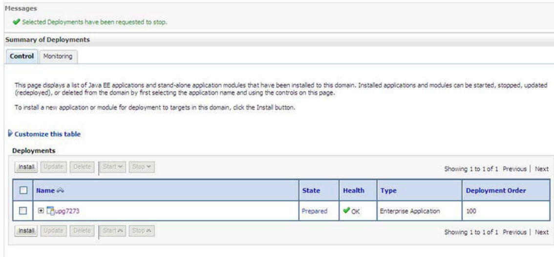
Figure 6–19 Summary of Deployments- Messages
