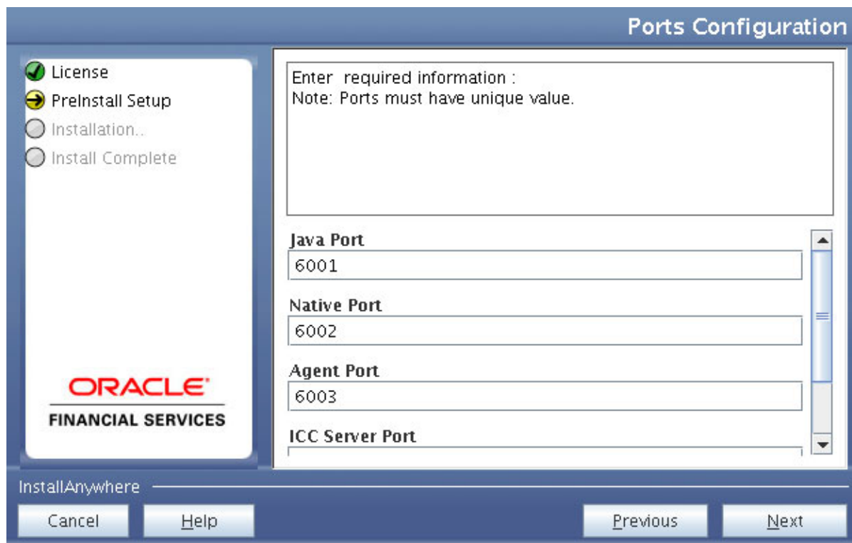
Figure 4–24 Ports Configuration
