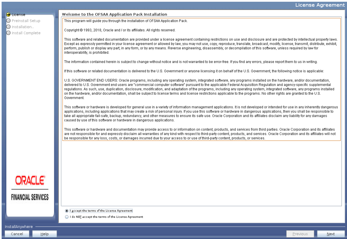
Figure 4–10 License Agreement
