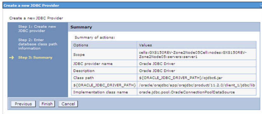
Figure 5–10 Summary
