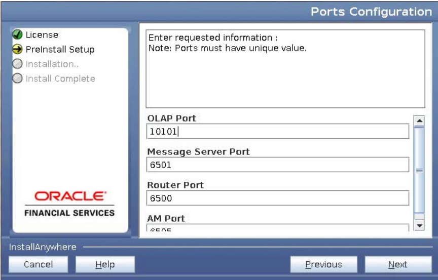
Figure 4-32 Ports Configuration
