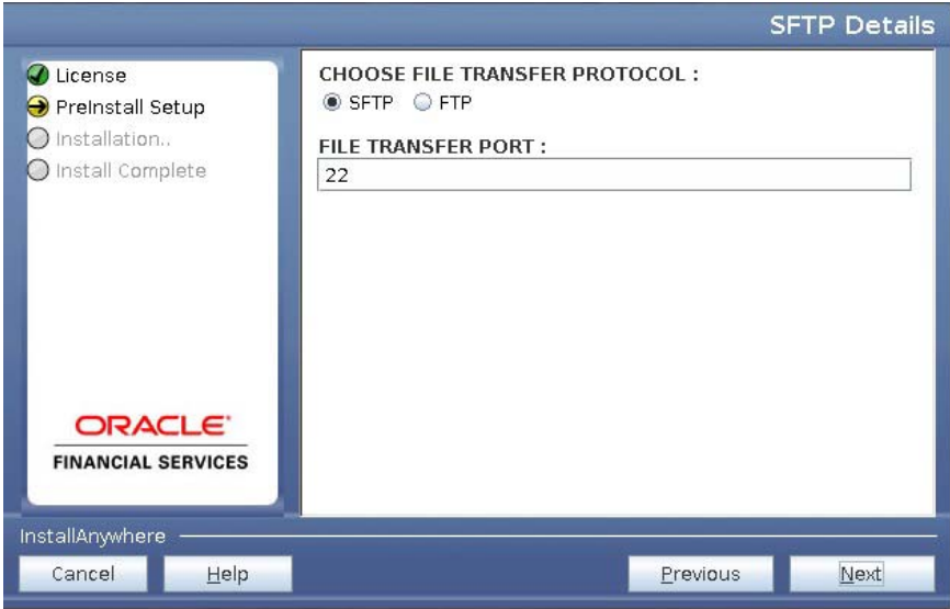
Figure 4-33 SFTP Details
