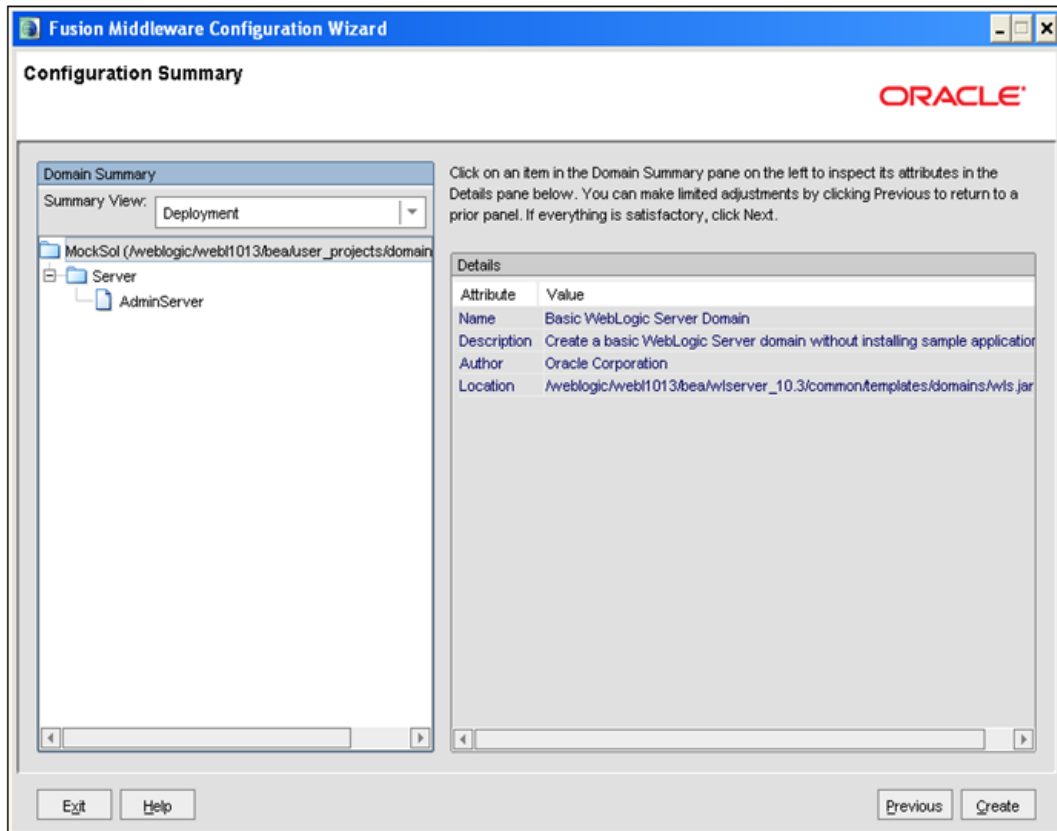
Figure 5–7 Configuration Summary
