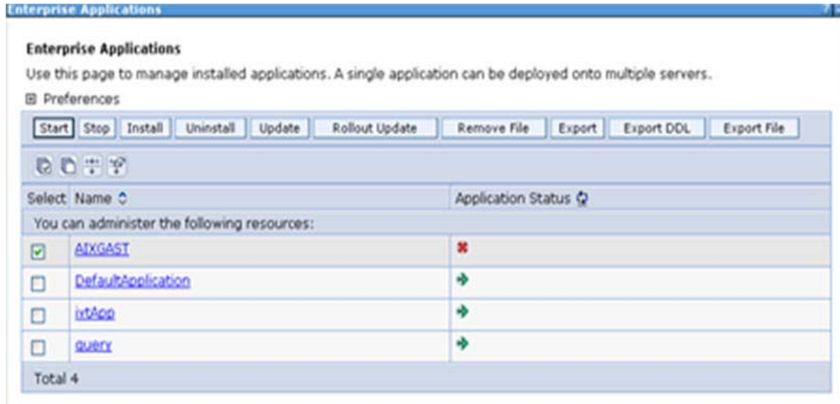
Figure 5–2 Enterprise Applications
