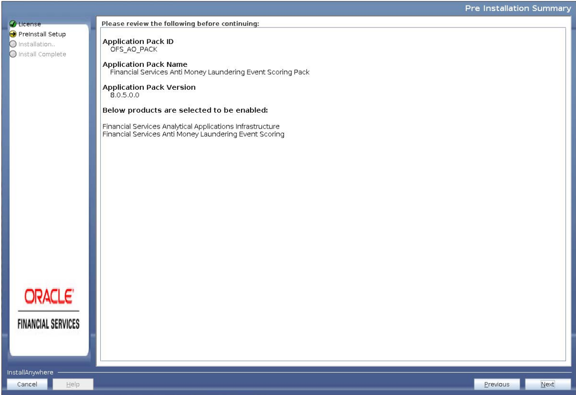
Figure 4-19 Pre-Installation Summary
