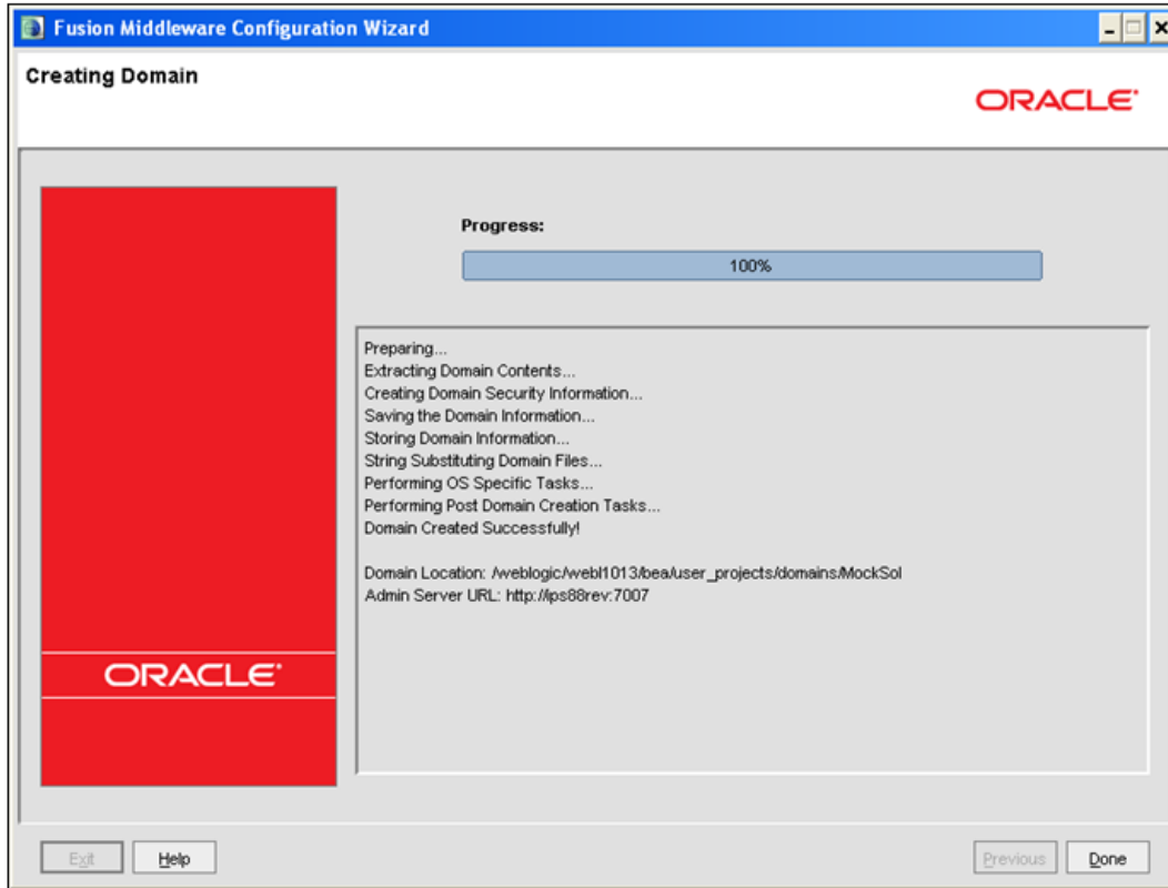
Figure 5–8 Creating Domain
