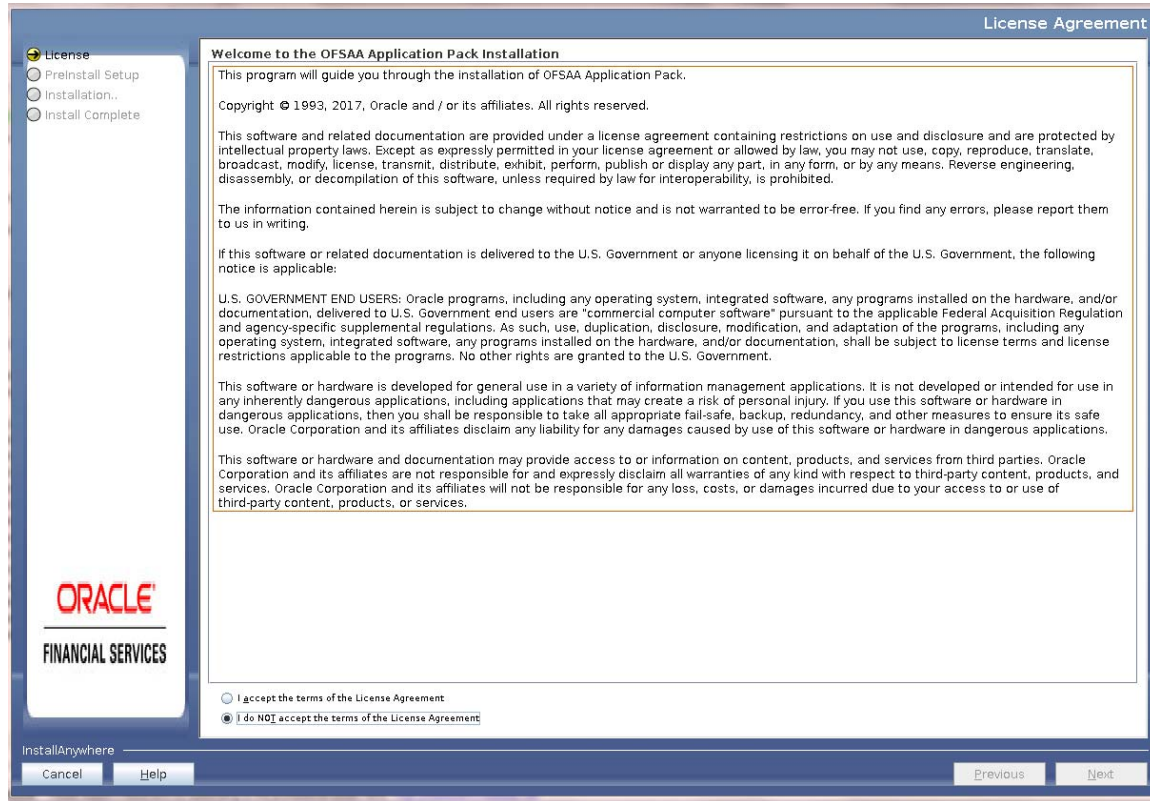
Figure 4–16 License Agreement
