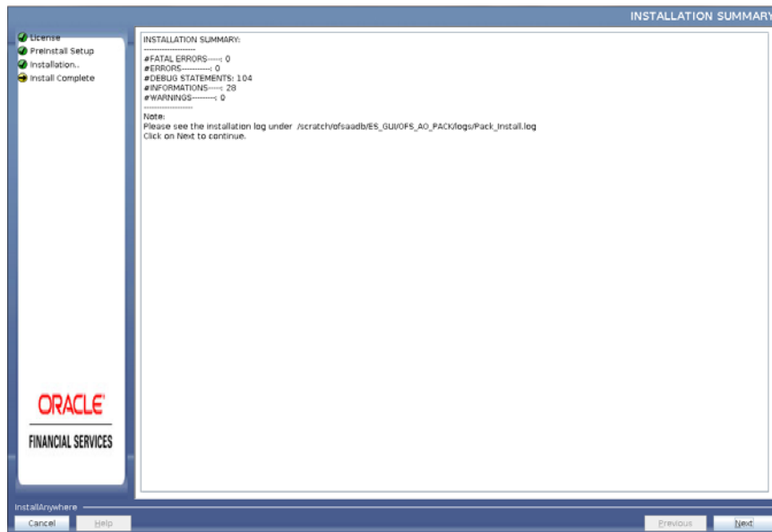
Figure 4–42 Installation Summary
