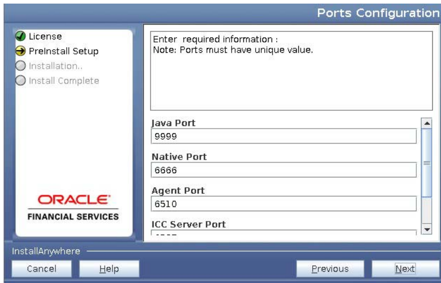
Figure 4–31 Ports Configuration
