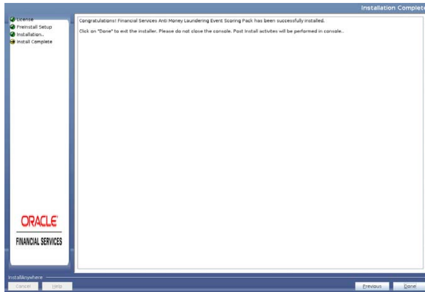
Figure 4–43 Installation Complete
