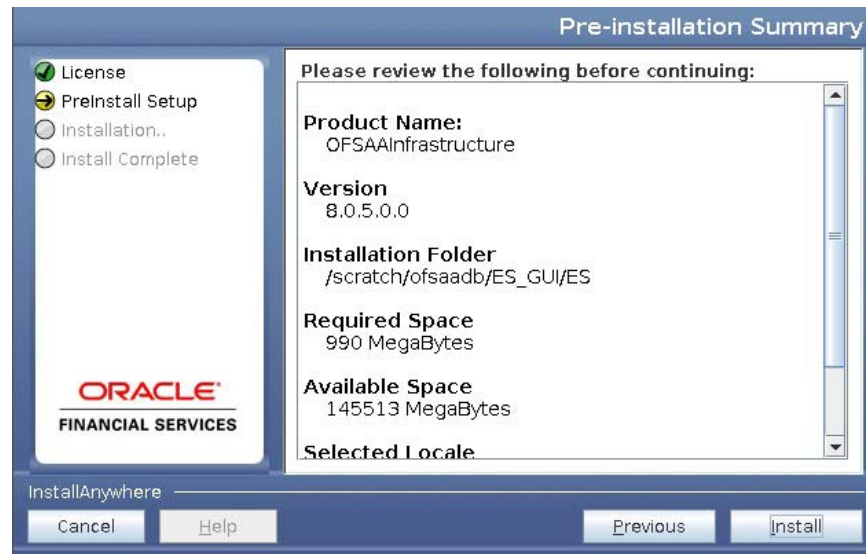
Figure 4–35 Pre-installation Summary
