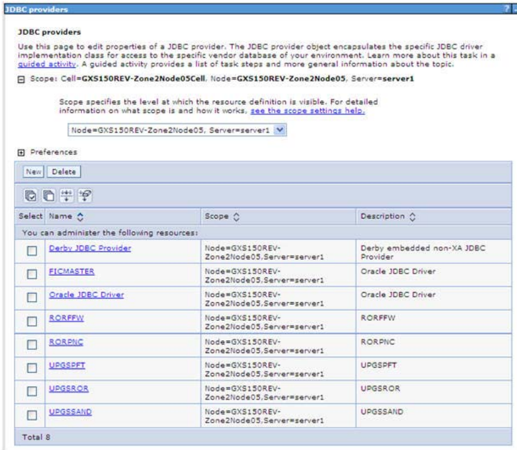
Figure 5–9 JDBC Providers
