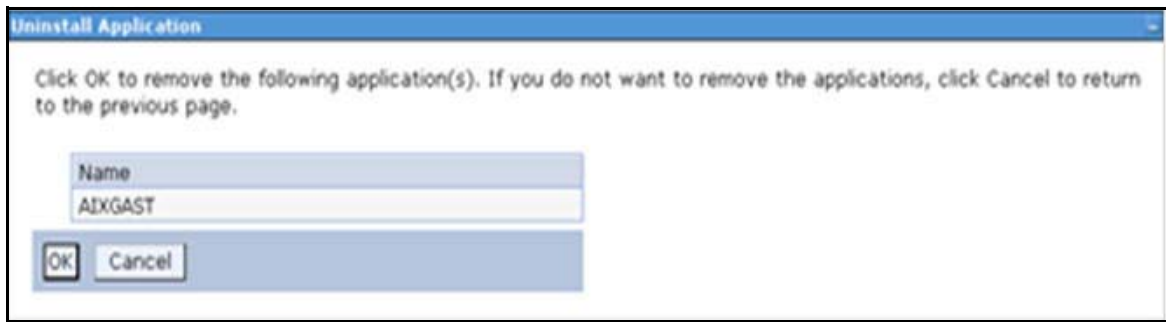
Figure 5–22 Uninstall Application
