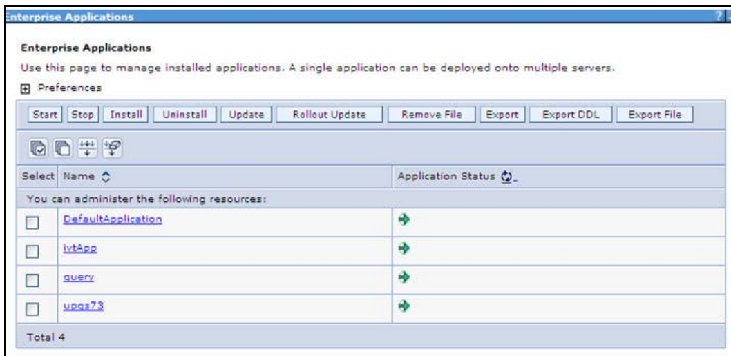
Figure 5–21 Enterprise Applications
