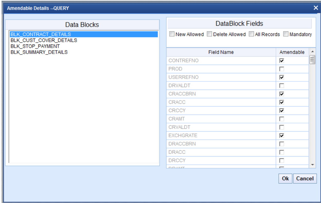
Fig 14.2 Maintaining Amendable Fields Information
