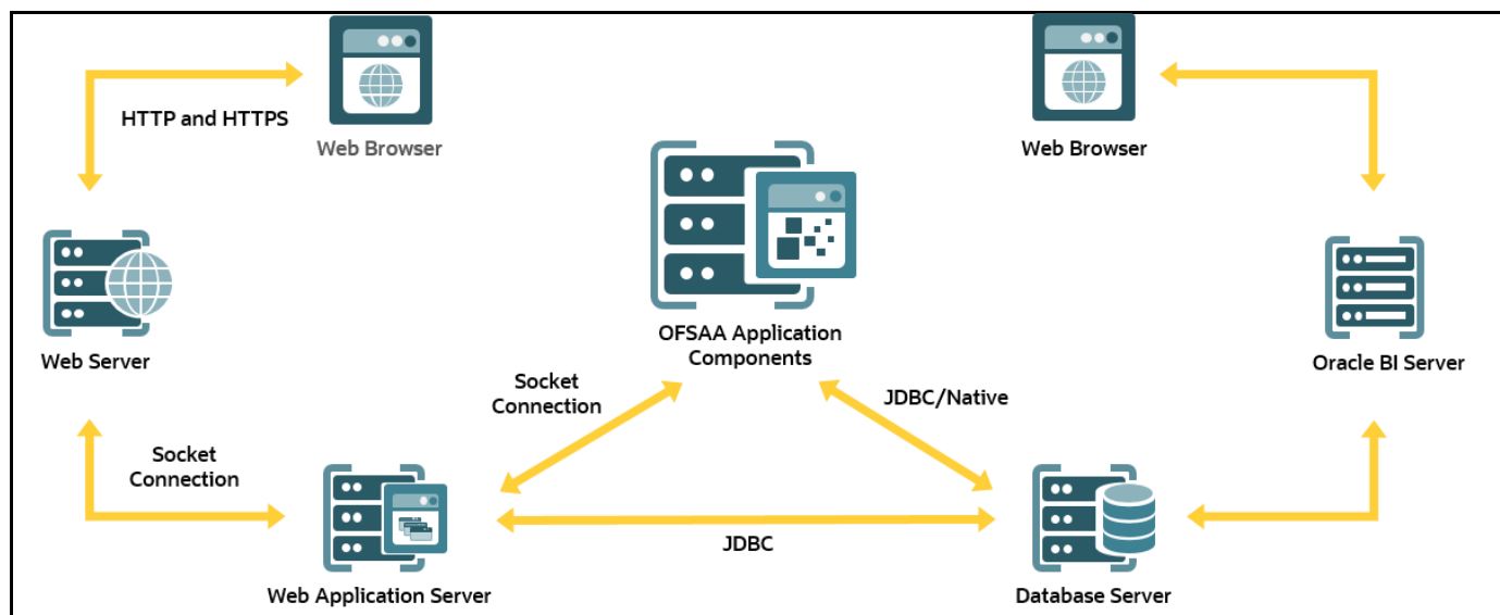
Figure 3: The logical architecture implemented in the OFSAAI Application Pack
