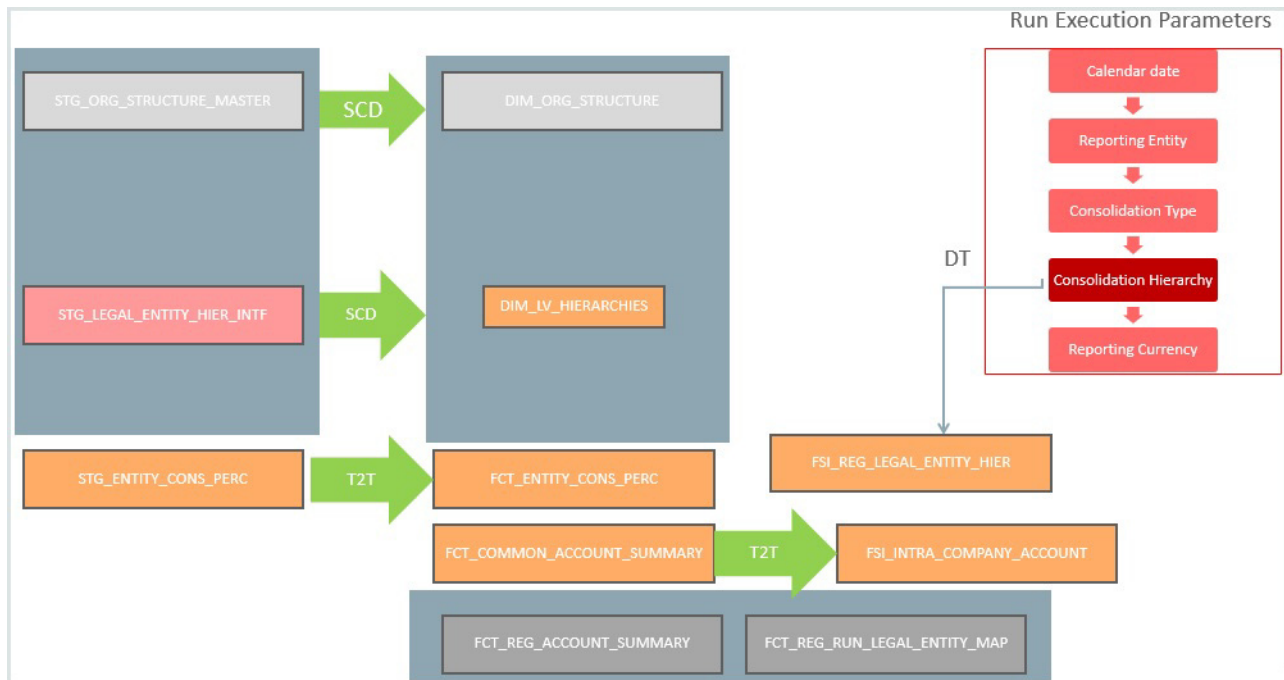
Figure 1. Data Flow
