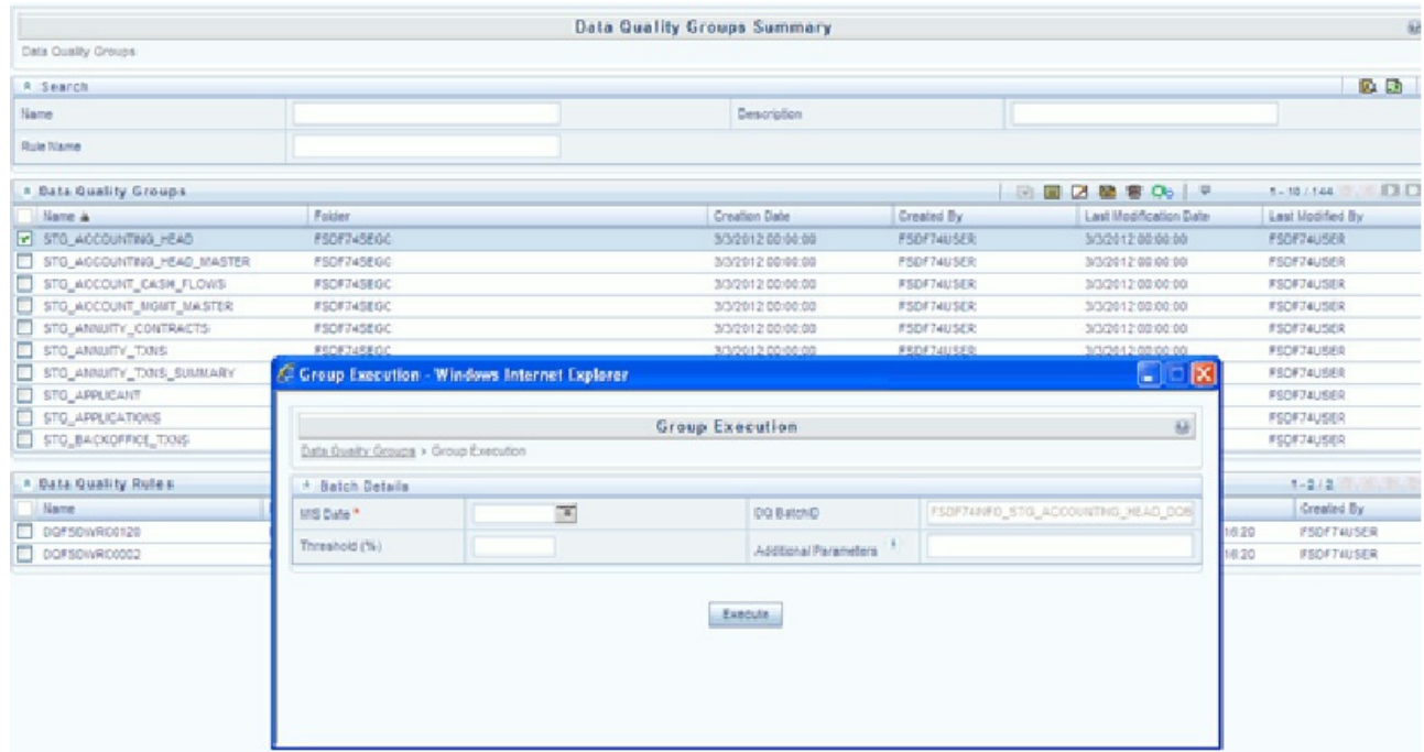
Figure 24. Group Execution
