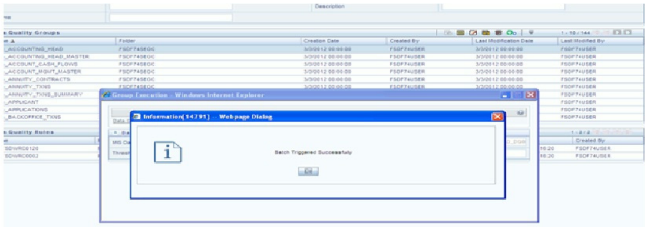
Figure 25. Execution Message
