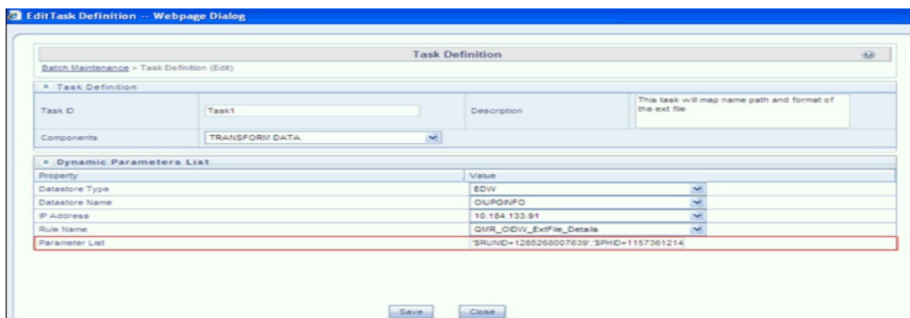
Figure 14. Task Definition
