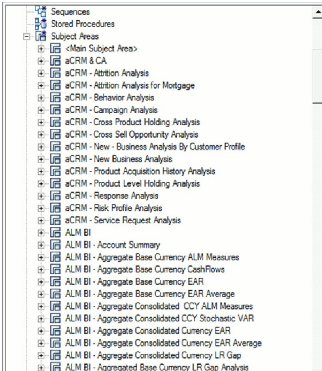
Figure 5. Subject Areas
