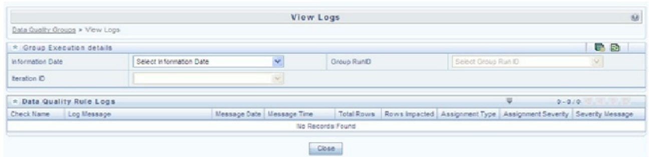
Figure 27. View Logs
