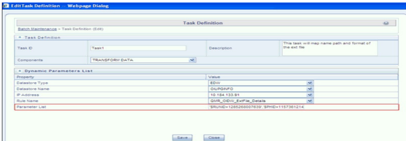
Figure 14. Task Definition
