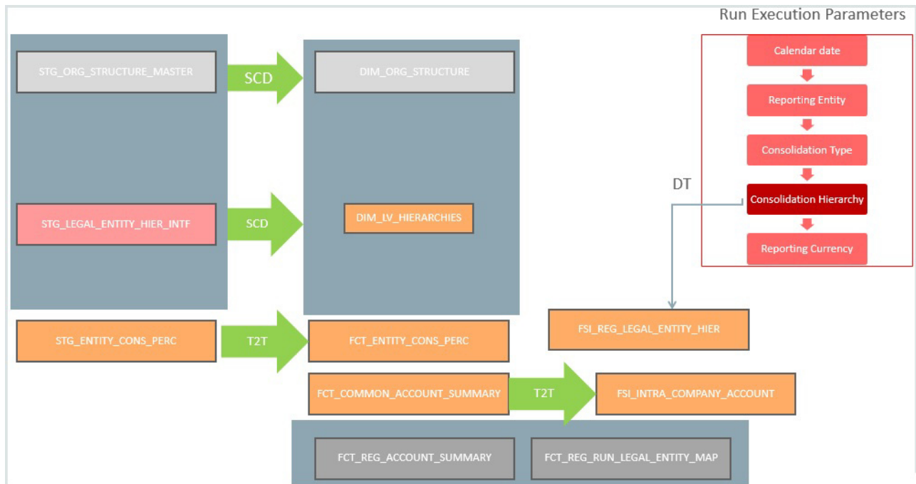
Figure 1. Data Flow
