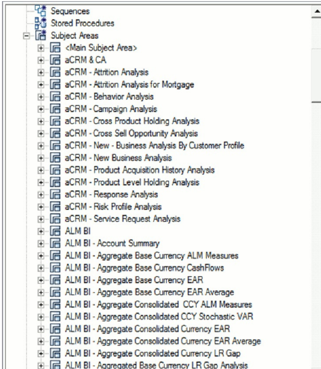
Figure 5. Subject Areas
