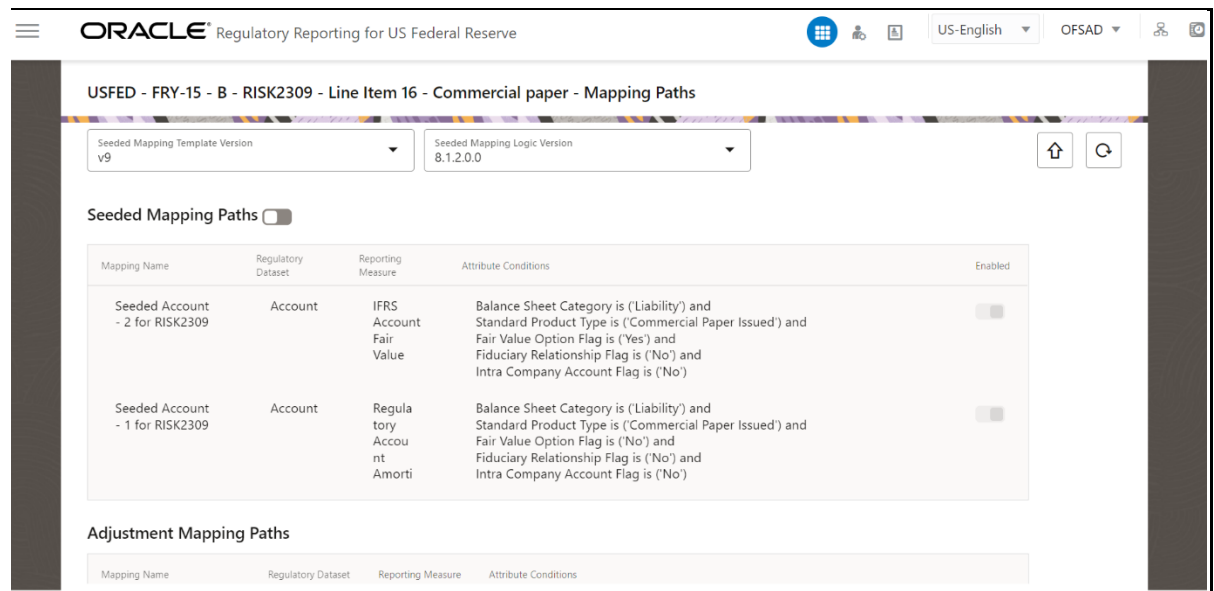
Figure 128: Disabled Seeding Mapping Details Page
