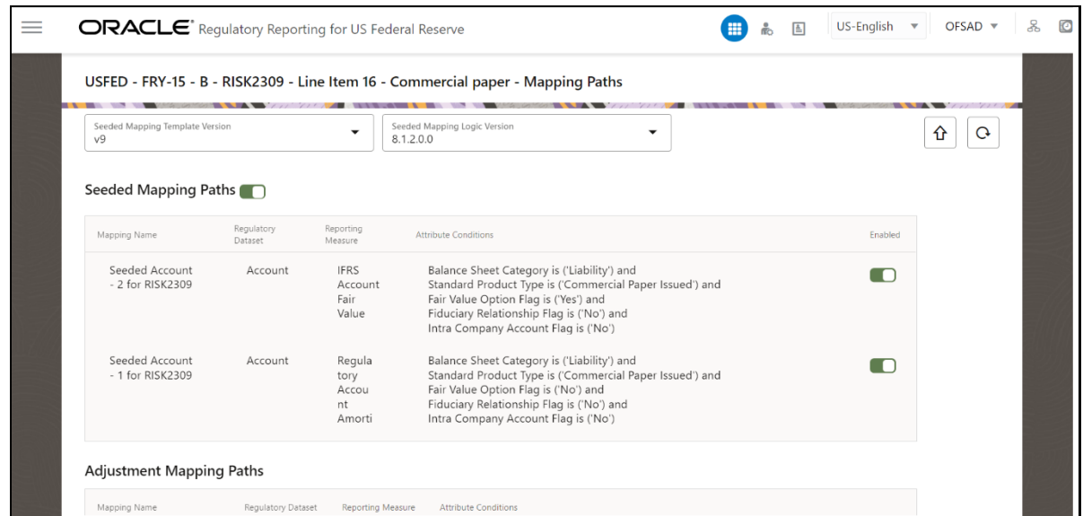
Figure 134: Seeded Mapping Details Page
