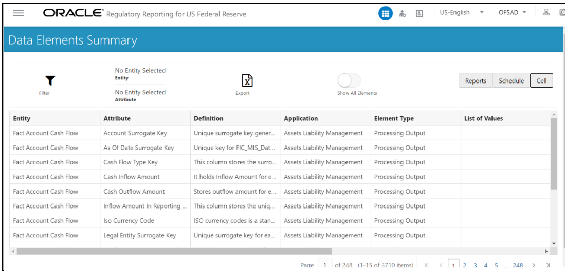
Figure 199: Data Elements Summary
