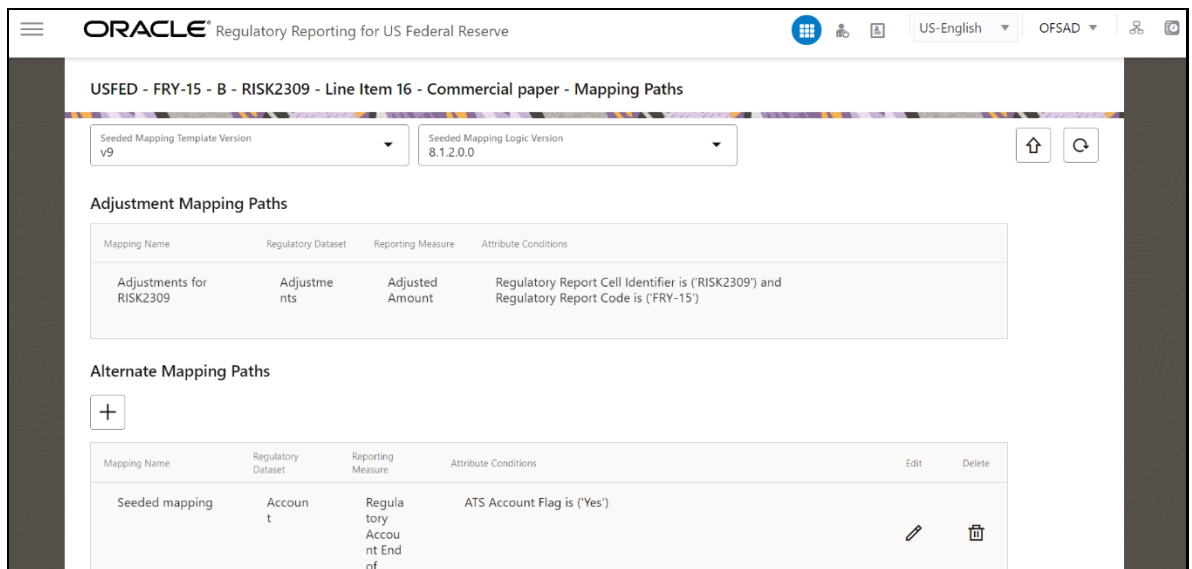
Figure 139: Added Mapping Save Page
