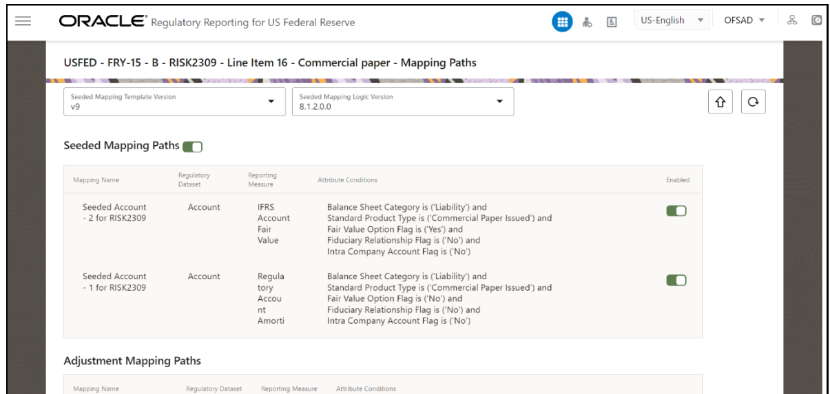
Figure 125: Seeded Mapping Details Page
