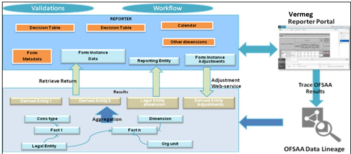
Figure 84: Data Flow between OFSAA and AgileREPORTER
