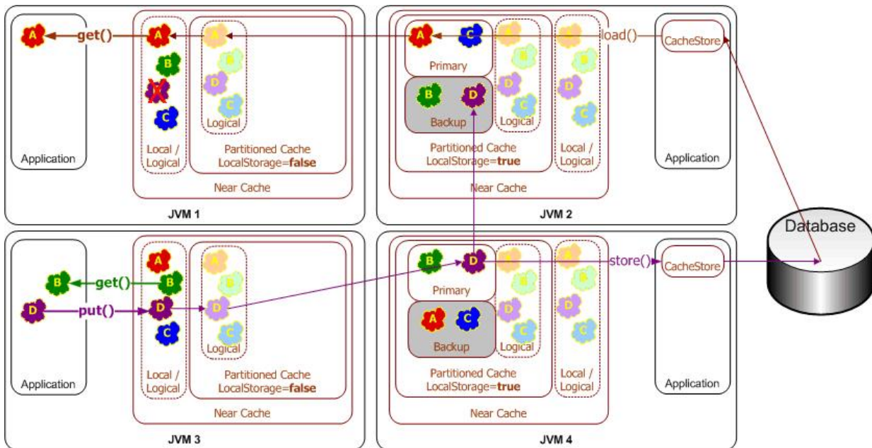
Figure 14-2 Write-Through Caching
