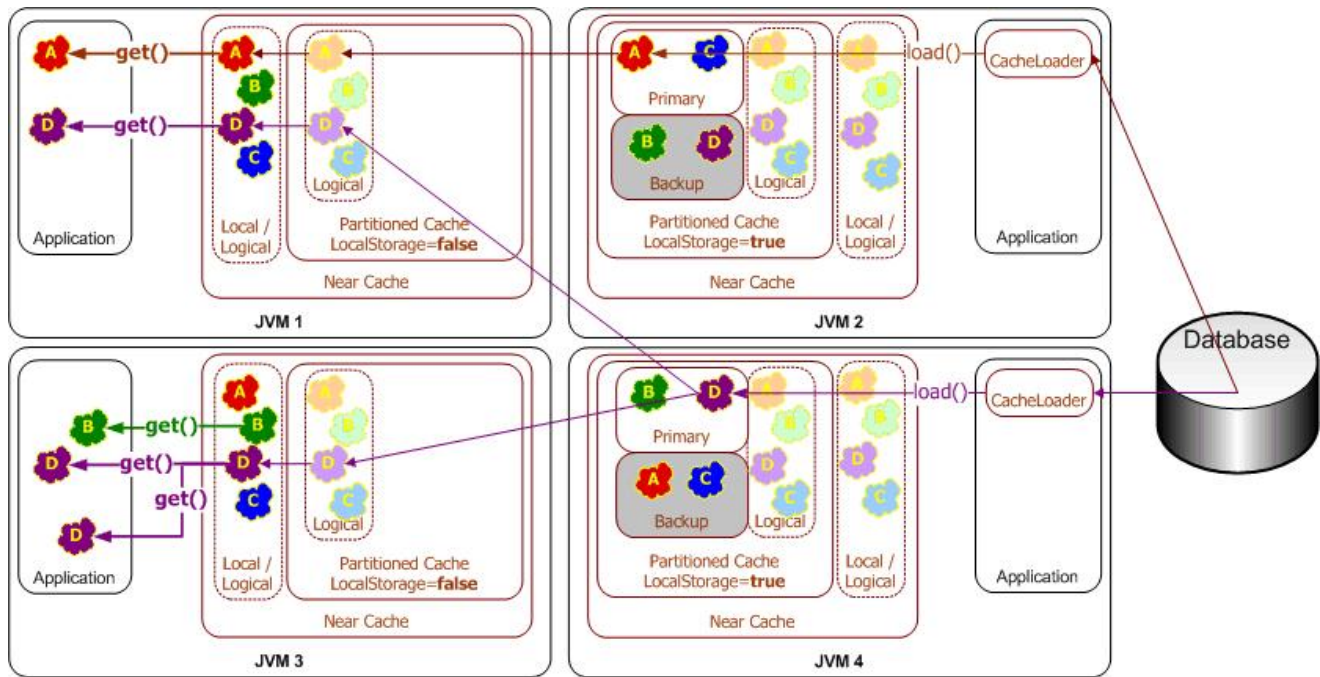
Figure 14-1 Read-Through Caching
