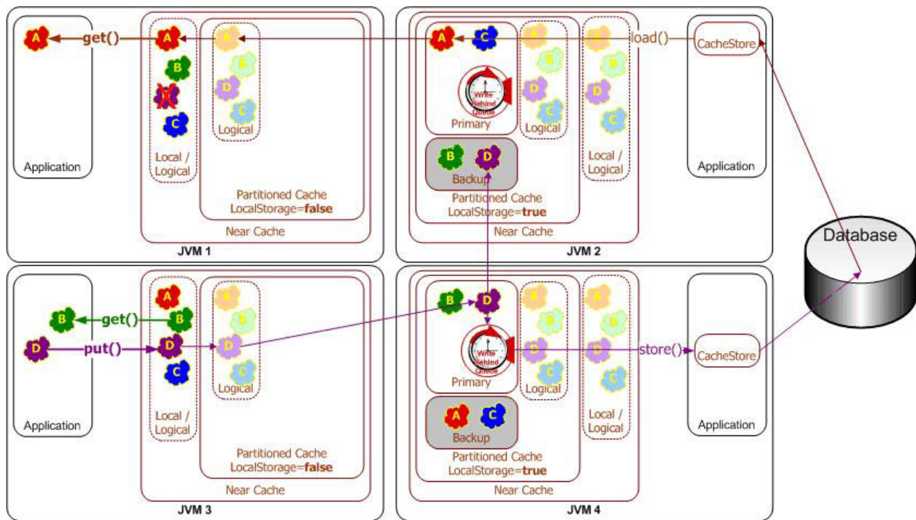
Figure 14-3 Write-Behind Caching
