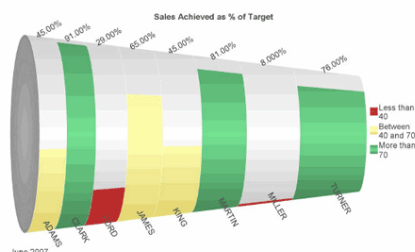
Figure 39–3 Funnel Graph
