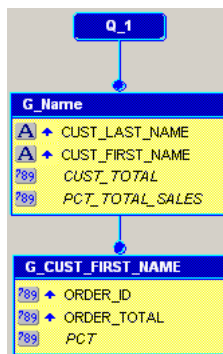
Figure 15–5 Data Model with Three Summary Columns
