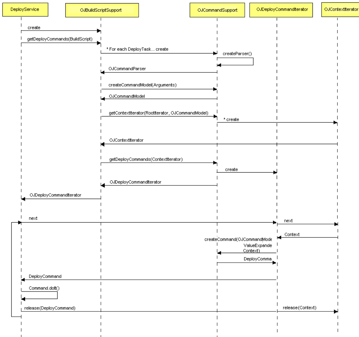
Figure 22-6 Sequence Diagram
