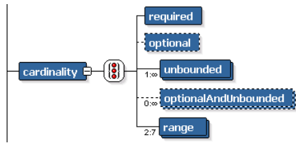
Figure 20-7 Cardinality Component
