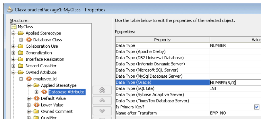
Figure 5-26 Database Attributes for Applied Stereotypes
