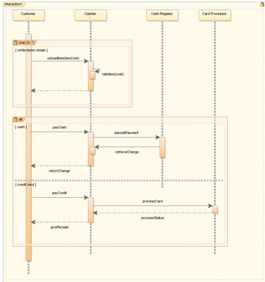
Figure 5-33 Typical Sequence Diagram with Combined Fragments
