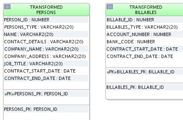
Figure 5-22 Transformed Root Classes
