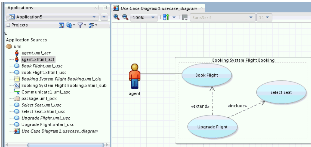
Figure 5-39 Exported Model
