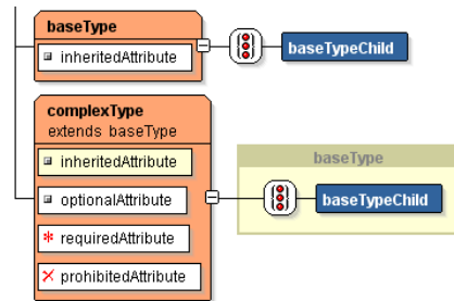
Figure 20-8 complexType Component
