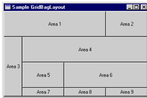
Figure 13-5 GridBagLayout
