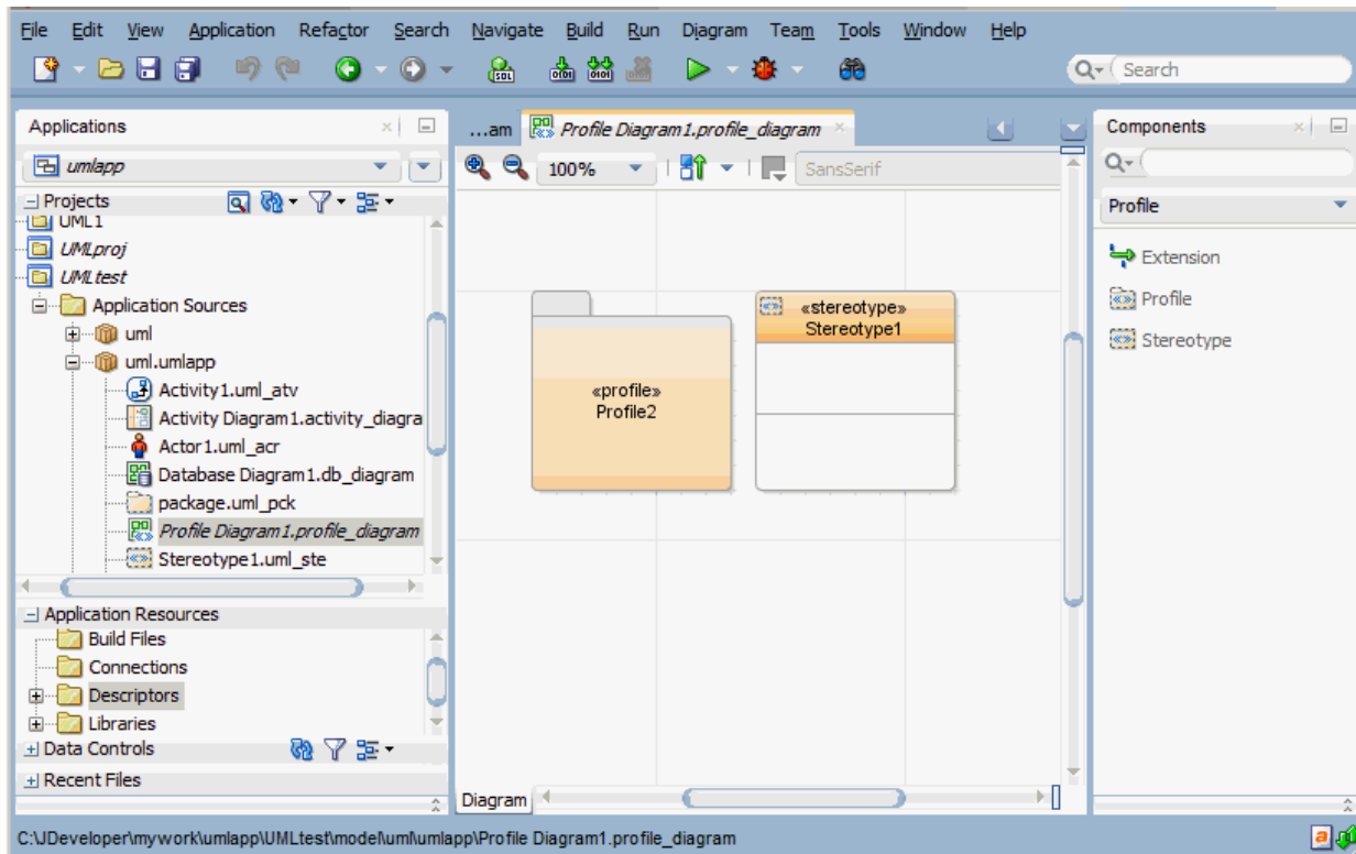
Figure 5-48 Profile Diagram
