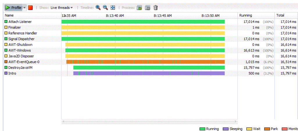
Figure 10-10 Threads Session
