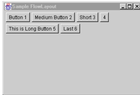
Figure 13-4 FlowLayout
