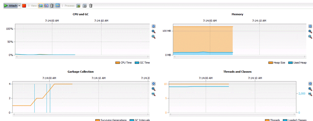
Figure 10-6 Telemetry Session
