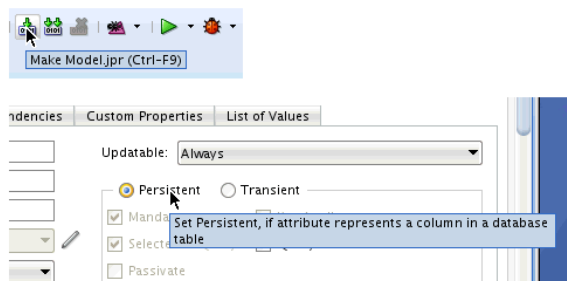
Figure 7-2 InfoTips
