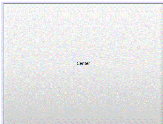
Figure 13-3 Card layout
