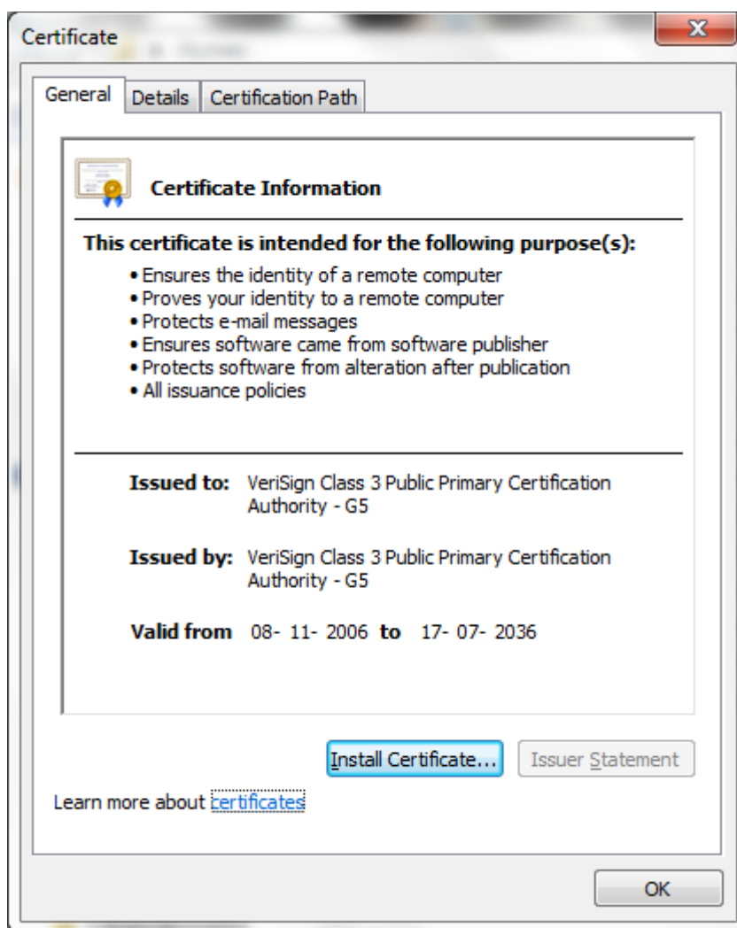
図 2-9 Certificate Information
