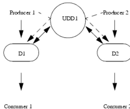
Figure 10-1 Paired Producers and Consumers
