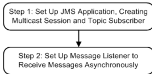
Figure 9-1 Setting Up Multicasting
