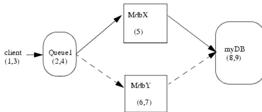
Figure 11-2 Workflow for Joe's Order Using Unit-of-Order
