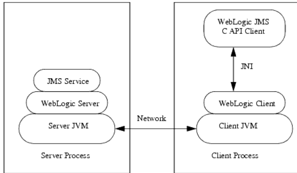
Figure 16-1 WebLogic JMS C API Client Application Environment
