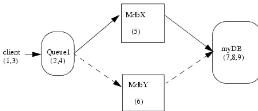
Figure 11-1 Workflow for Joe's Order
