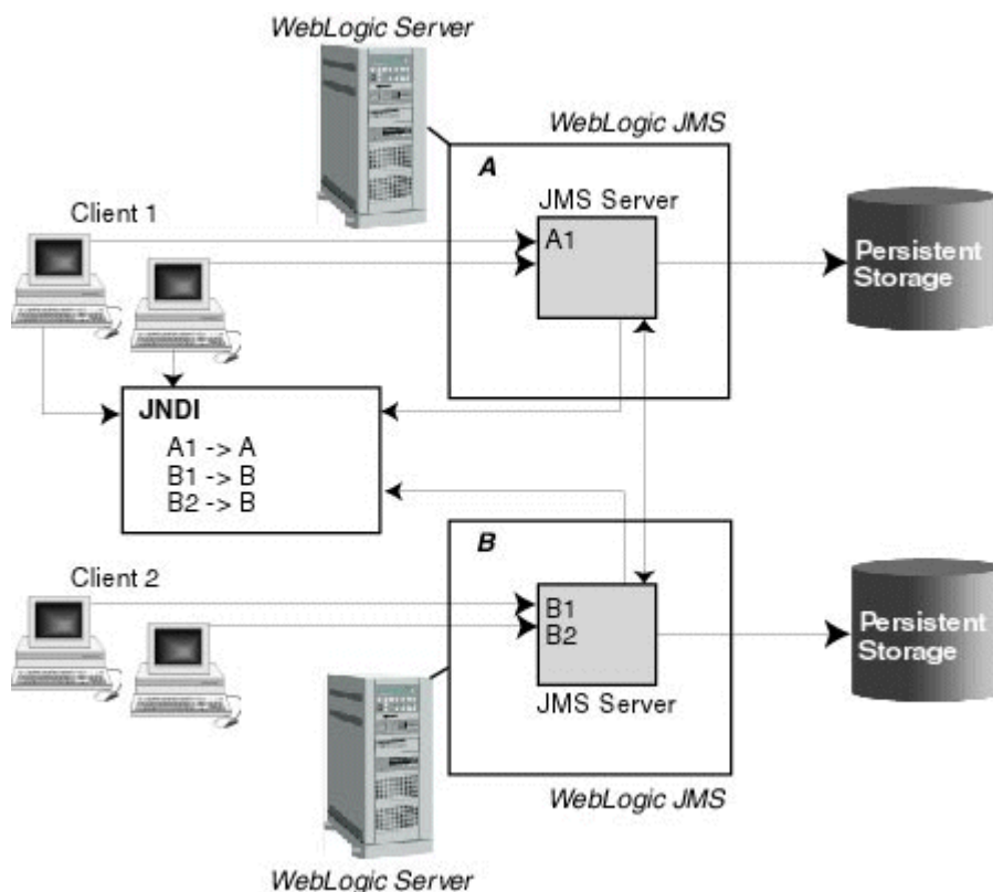
Figure 2-2 WebLogic JMS Architecture
