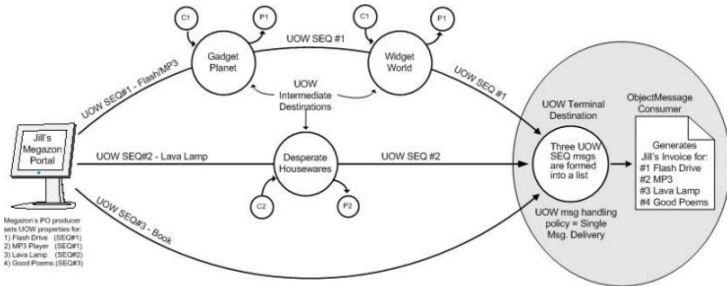
Figure 12-1 Workflow for Jill's Order Using Unit-of-Work
