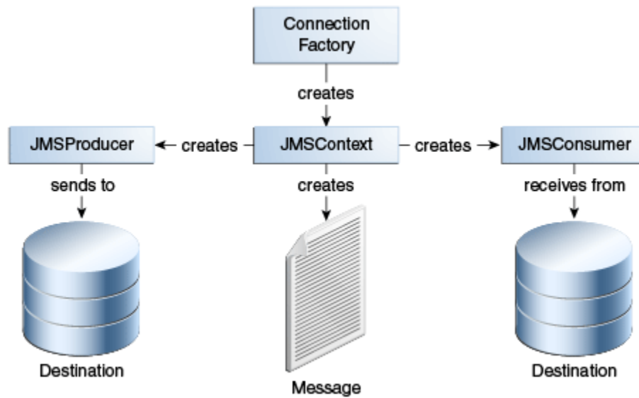
Figure 5-1 Simplified API Programming Model
