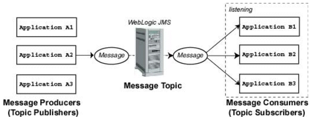
Figure 2-4 Publish/Subscribe Messaging
