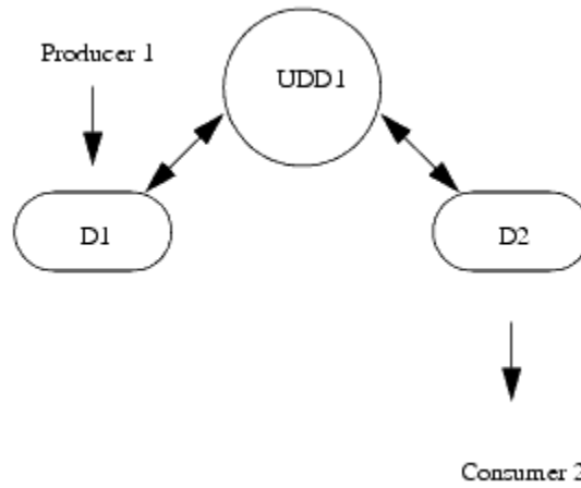
Figure 10-3 Stuck Messages
