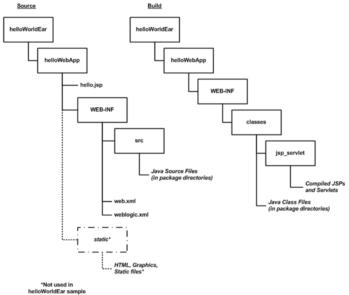
Figure 4-5 Web Application Source and Build Directories
