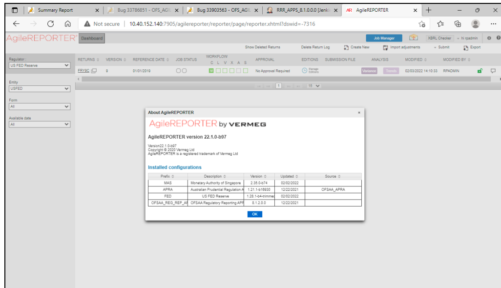
Figure 24: AgileREPORTER Dashboard
