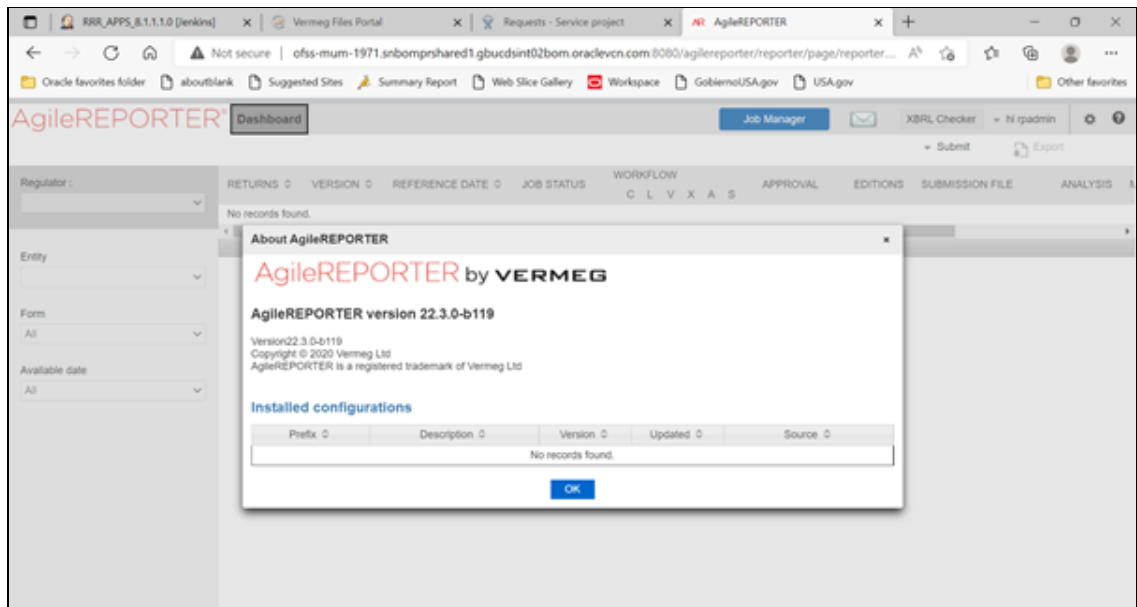
Figure 24: AgileREPORTER Dashboard
