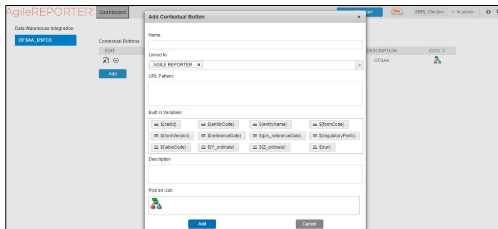
Figure 39: Adding Contextual Button
