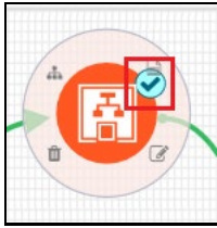
Figure 106: Sub Pipeline
