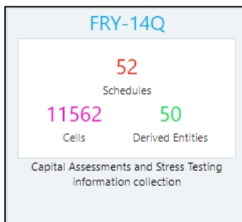
Figure 82: Report Information
