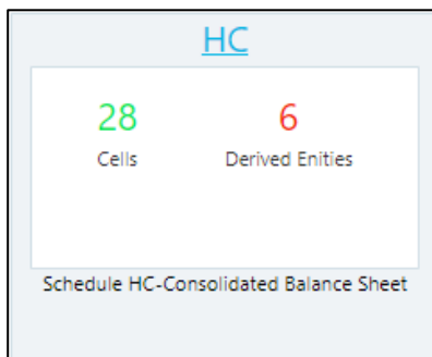
Figure 73: Schedule Information
