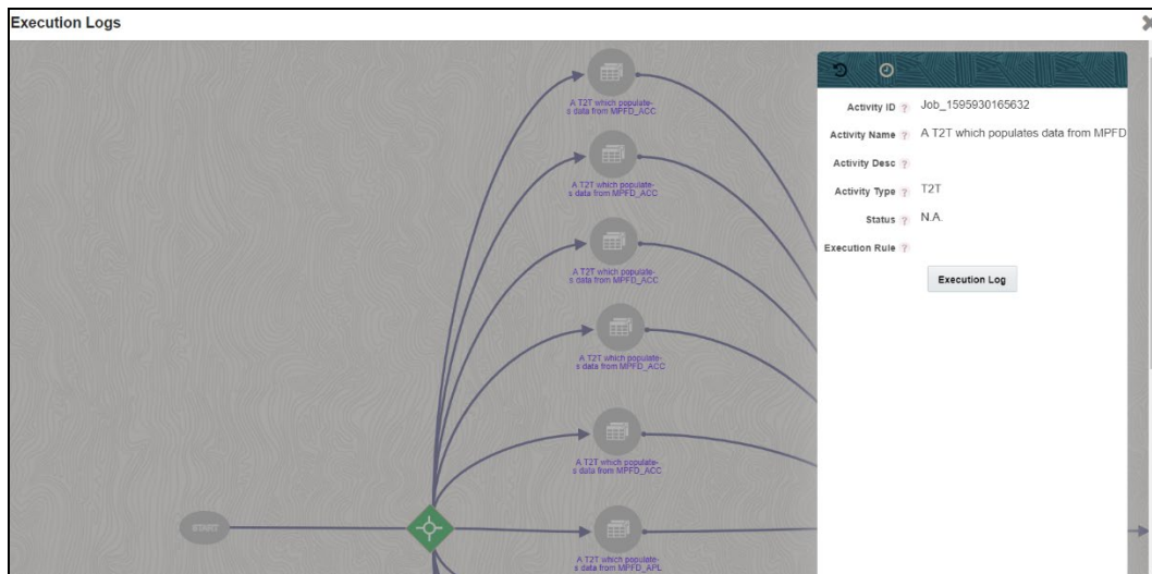
Figure 108: Activity Logs
