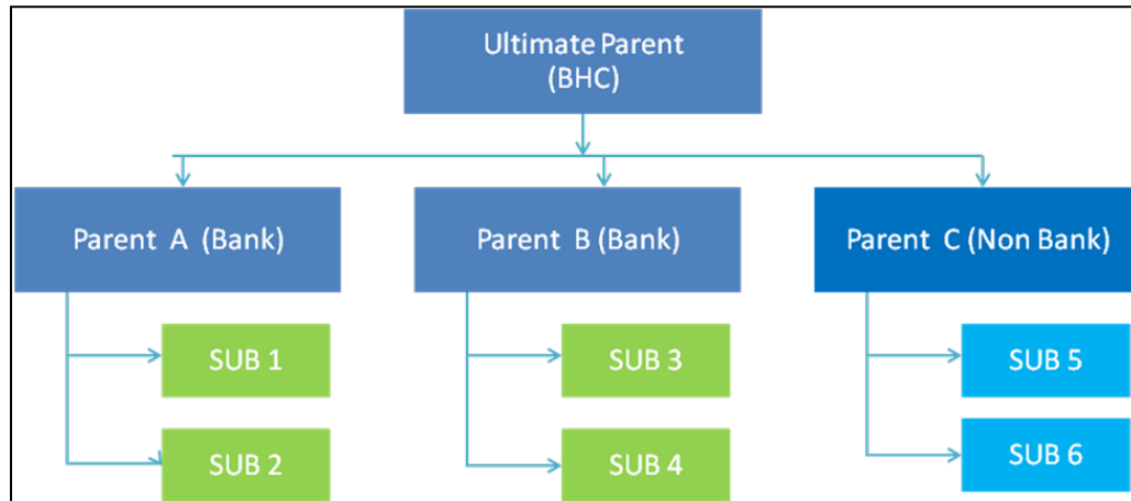
Figure 56: Consolidation workflow
