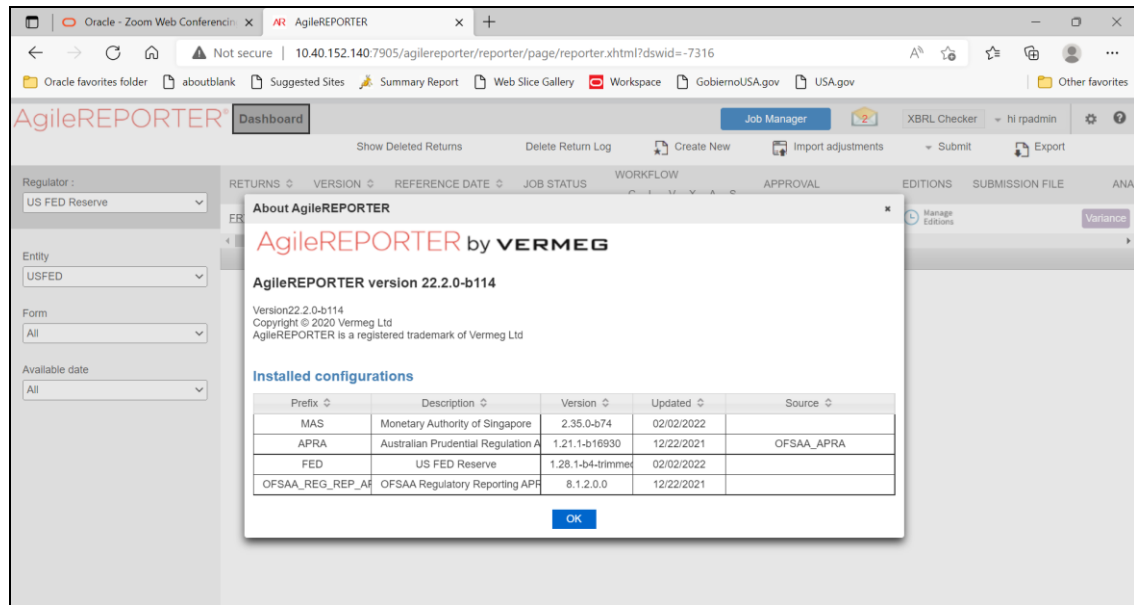
Figure 24: AgileREPORTER Dashboard
