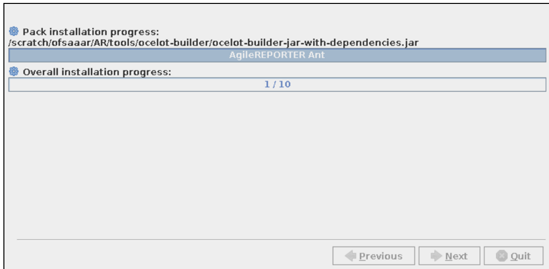
Figure 21: Installation progress Screen
