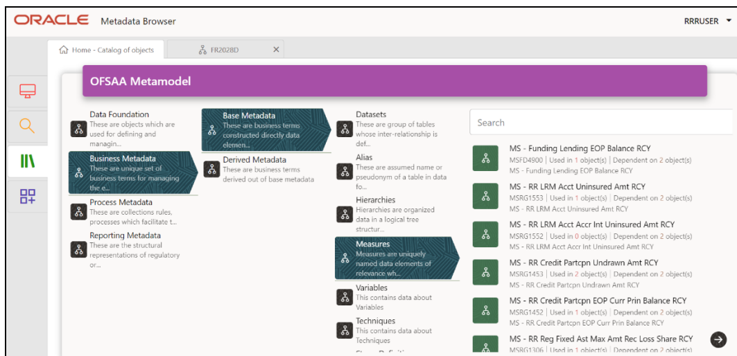
Figure 182: MDB - Business Metadata - Measure View Page
