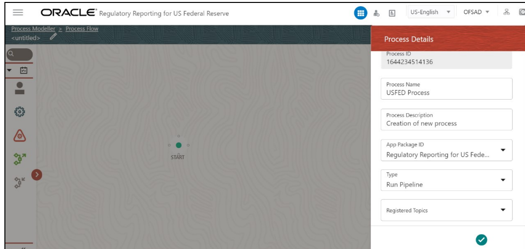
Figure 117: Updated Process Details Page
