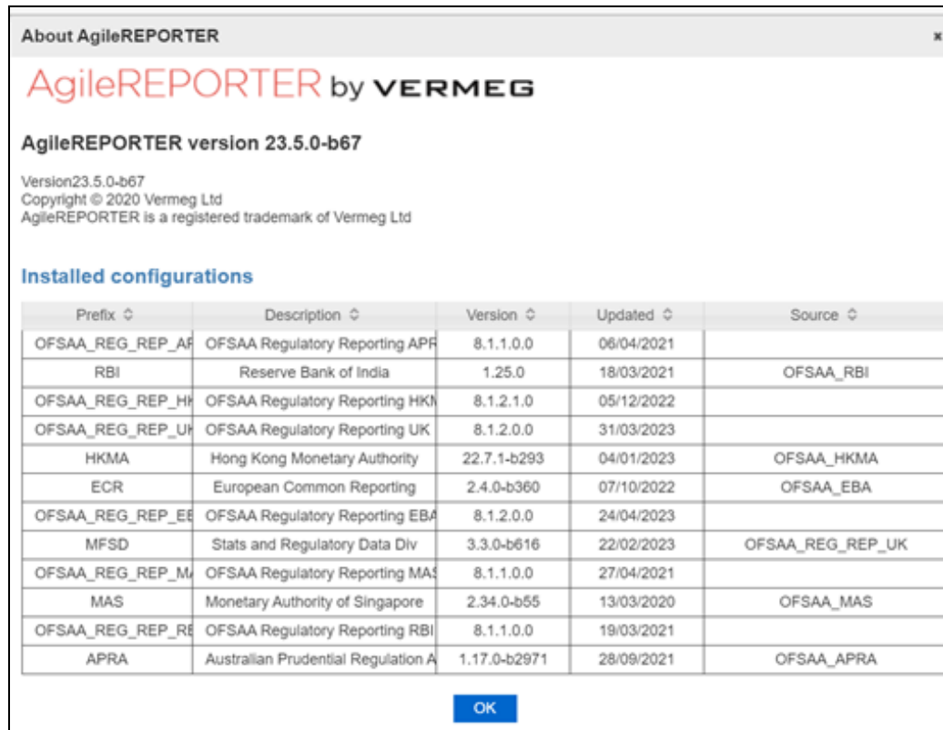
Figure 24: AgileREPORTER Dashboard
