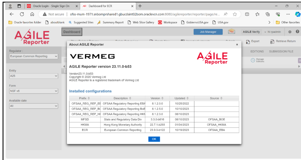
Figure 24: AgileREPORTER Dashboard
