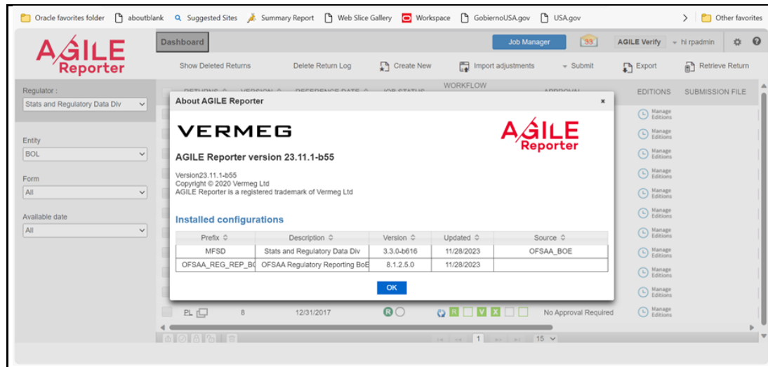
Figure 24: AgileREPORTER Dashboard
