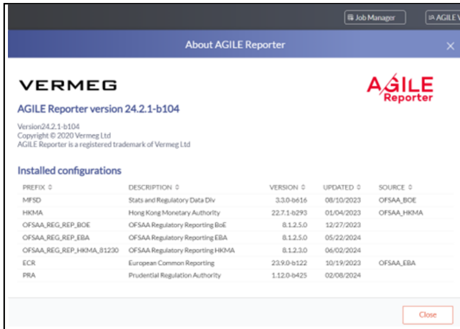
Figure 24: AgileREPORTER Dashboard
