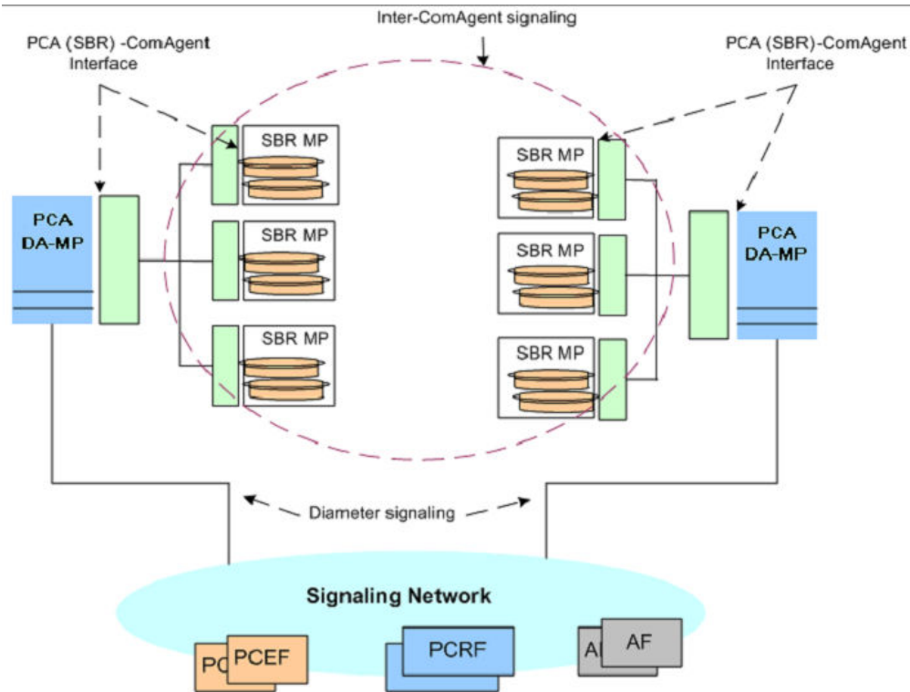
Figure 3-16 Communication between ComAgents, Policy DRA, and SBR
