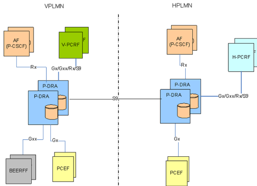
Figure 3-4 Policy DRA in Roaming Scenarios
