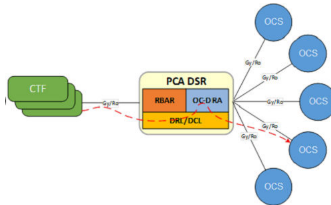
Figure 5-1 Local OCS Server Selection
