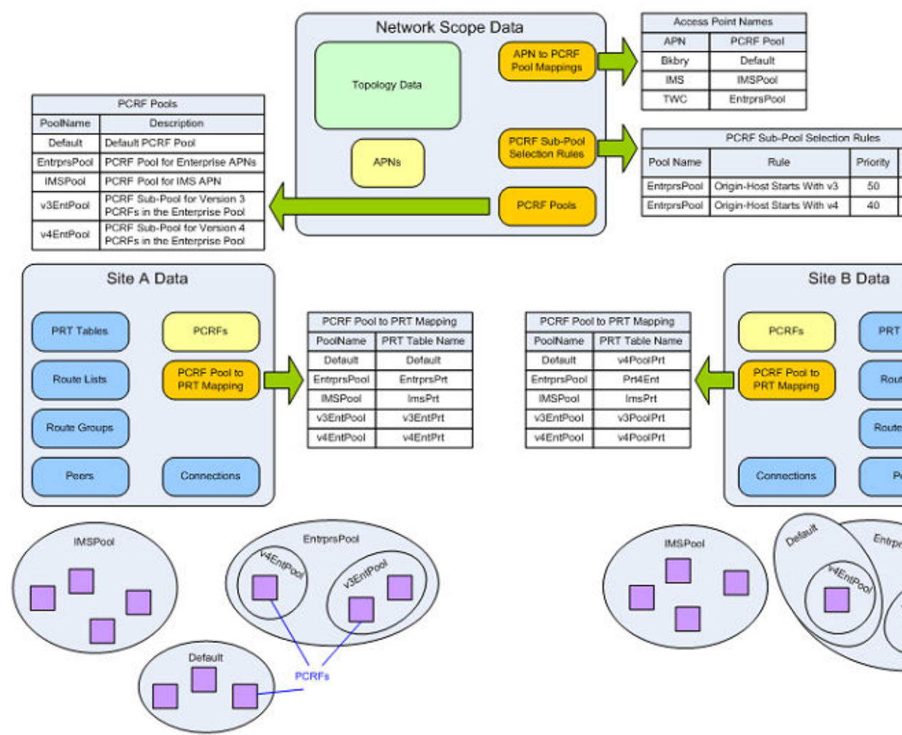
Figure 6-2 PCRF Pooling Data
