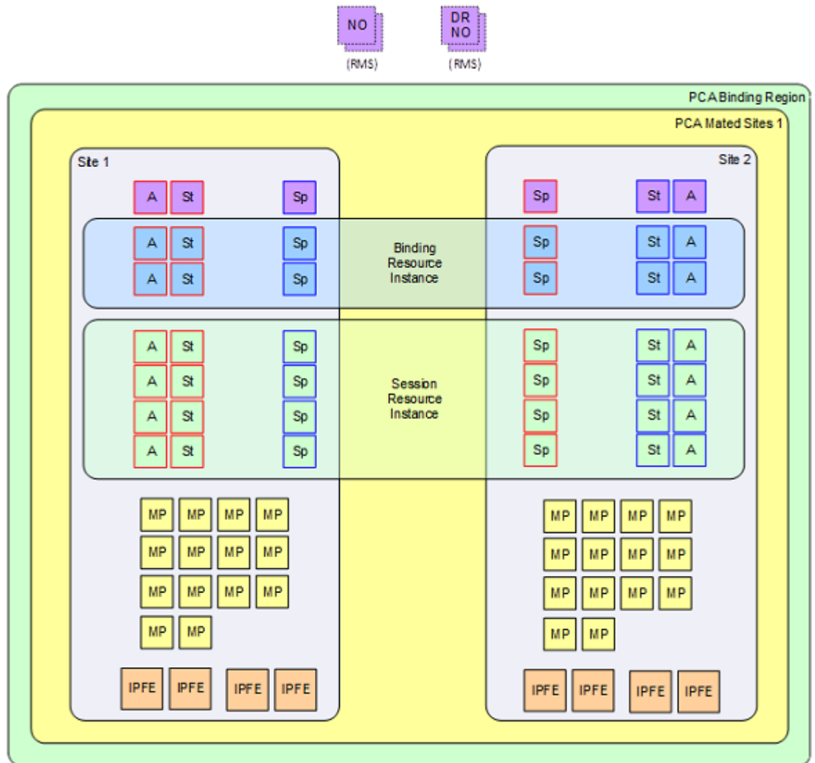
Figure 3-5 Example PCA Mated Pair - Hosting Binding SBRs
