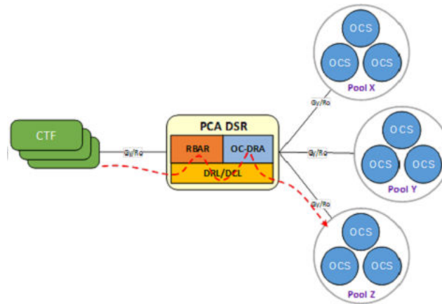
Figure 5-2 Local OCS Server Pool Selection
