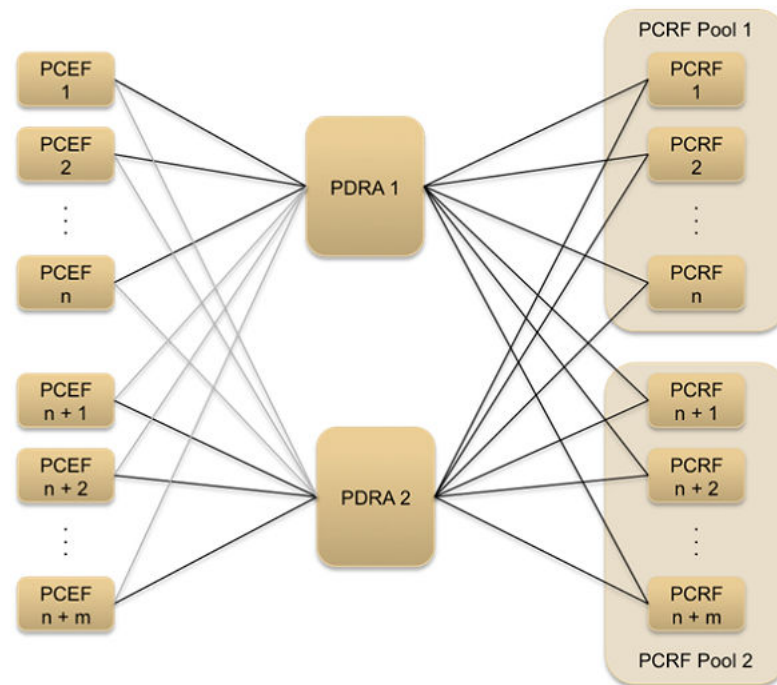
Figure 4-3 Multiple PCRF Pools
