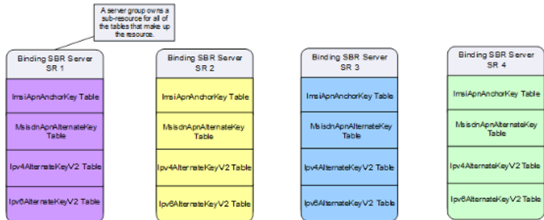
Figure 3-13 Multi-Table Resources
