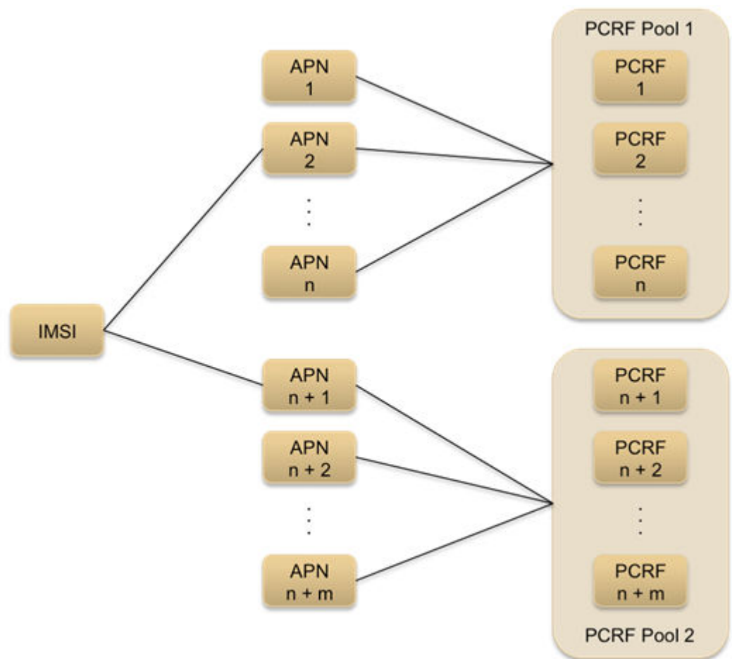
Figure 4-2 Relationship between IMSIs and PCRF Pools
