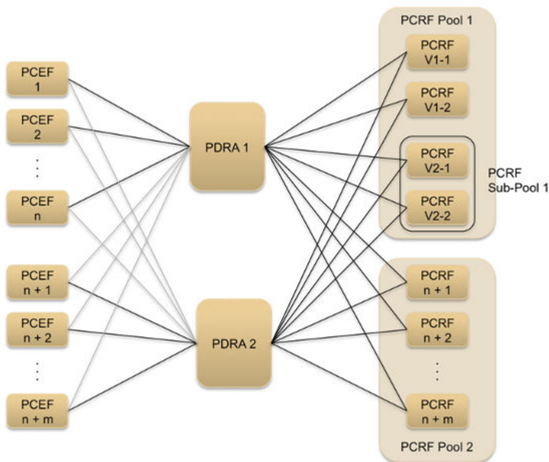
Figure 4-4 Multiple PCRF Versions in a PCRF Pool
