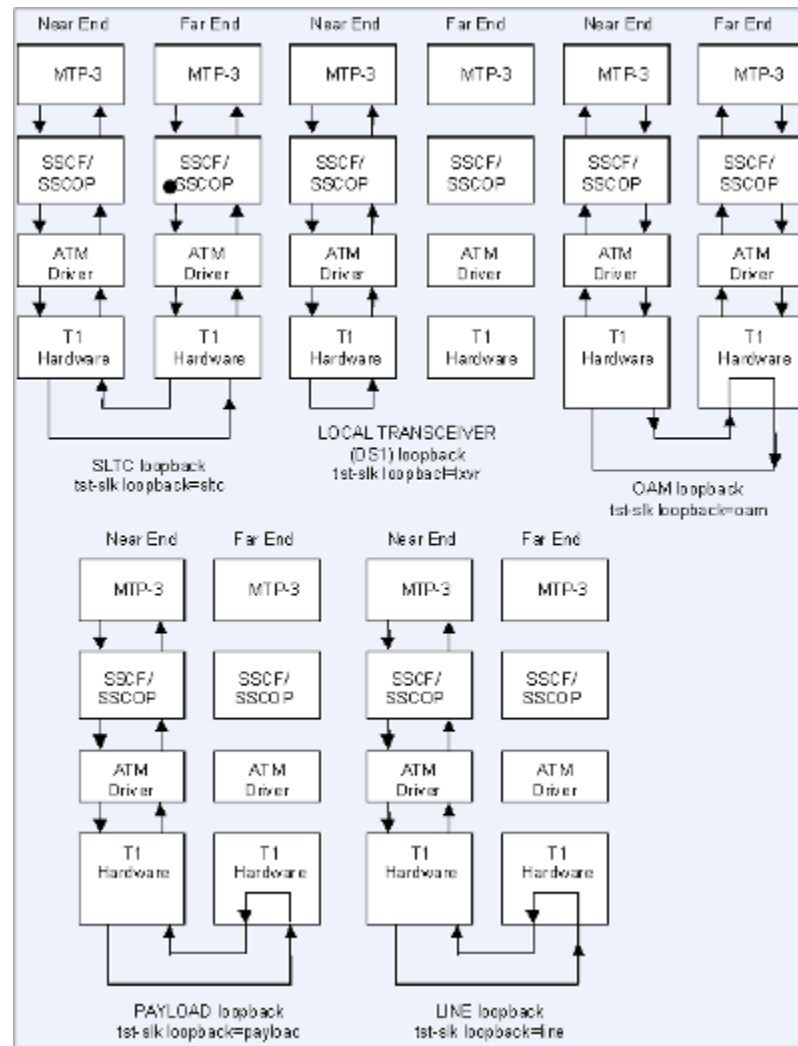
Figure A-1 ATM Loopback Tests
