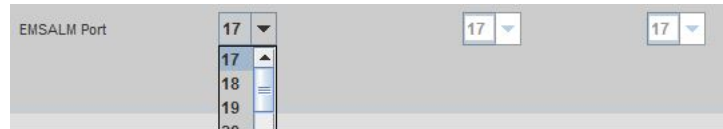
Figure 5-13 EMSALM Ports
