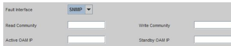
Figure 5-14 SNMP Interface
