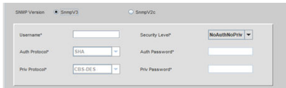
Figure 5-16 SnmpV3
