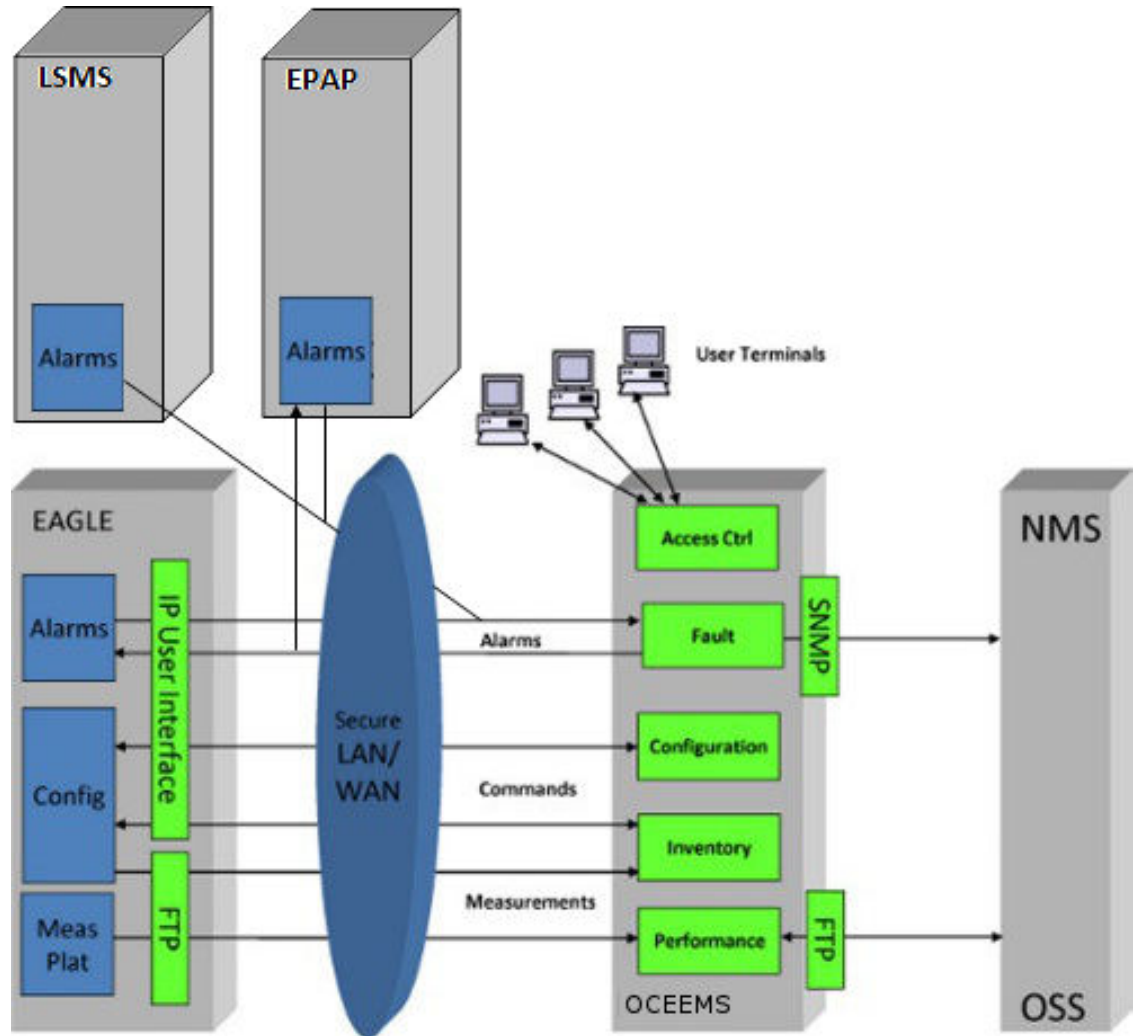
Figure 3-1 OCEEMS Architecture
