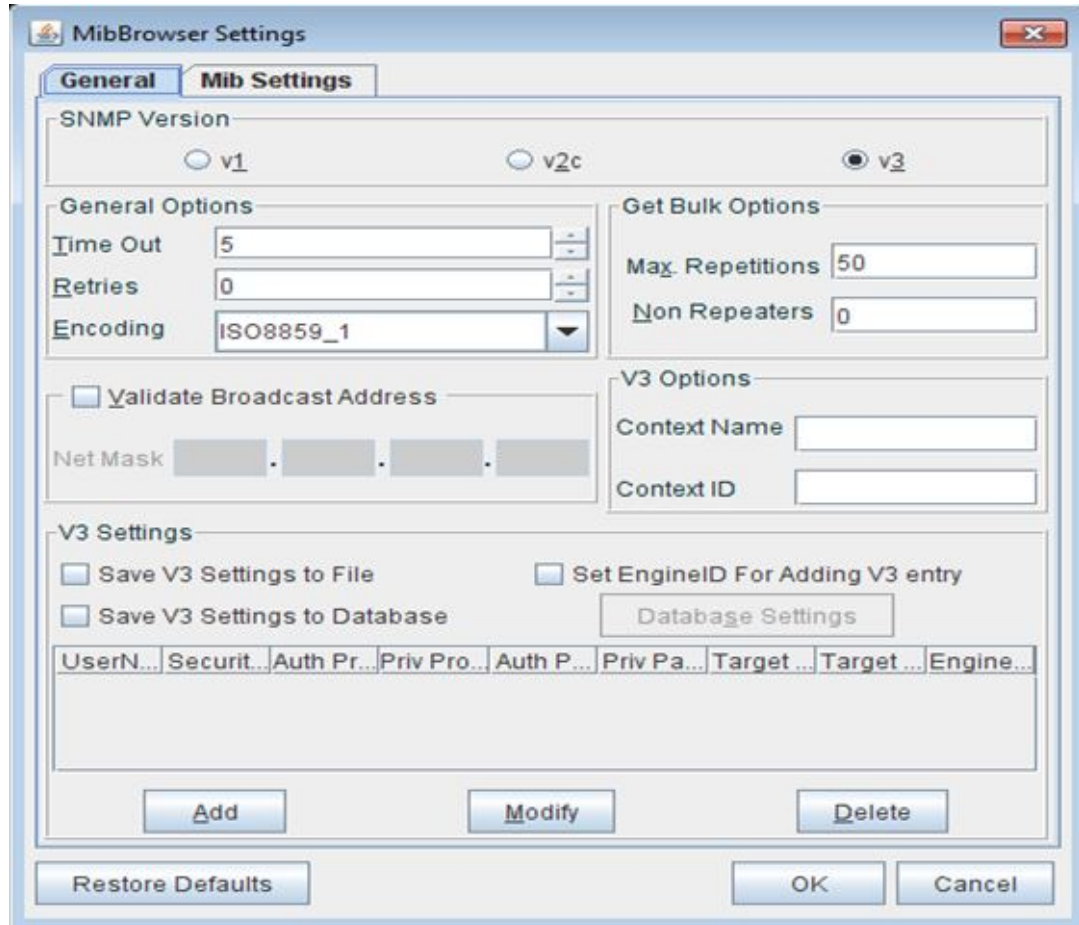
Figure G-2 MIB Browser Settings for v3
