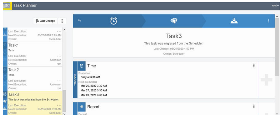
Figure 10-11 Task Planner
