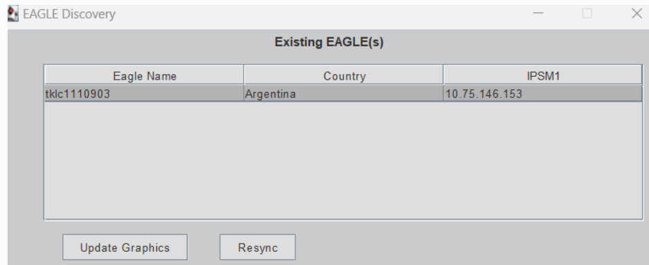
Figure 5-1 Eagle Discovery
