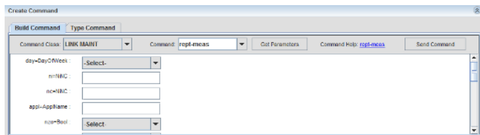
Figure 11-8 Get Parameters
