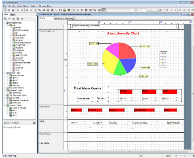
Figure 10-12 Report Designer
