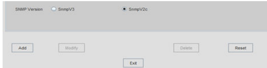
Figure 5-15 SnmpV2c
