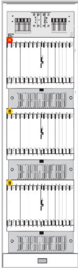
Figure 5-23 Chassis View
