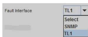
Figure 5-12 Fault Interface
