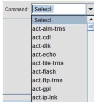
Figure 11-7 Command Menu
