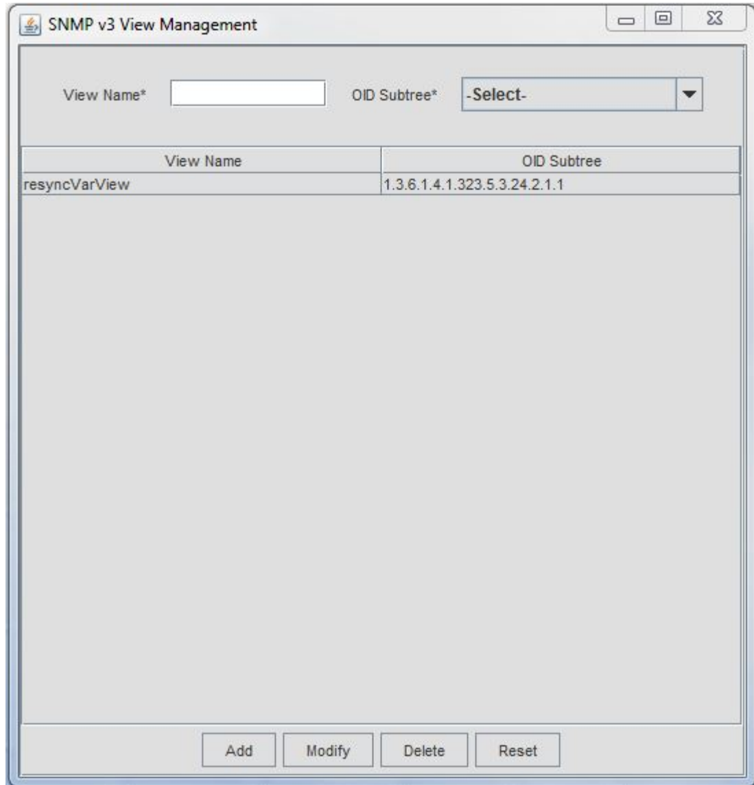
Figure 13-1 Sample SNMP v3 View Management Screen
