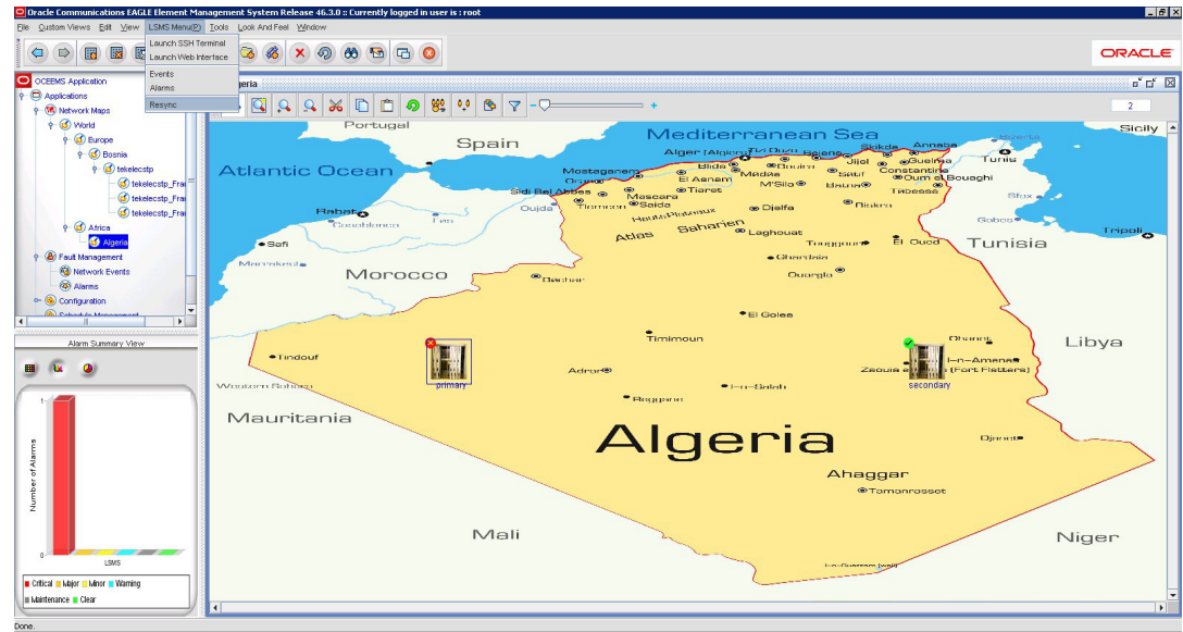
Figure 7-19 LSMS Resync Option in Maps - Menu Bar
