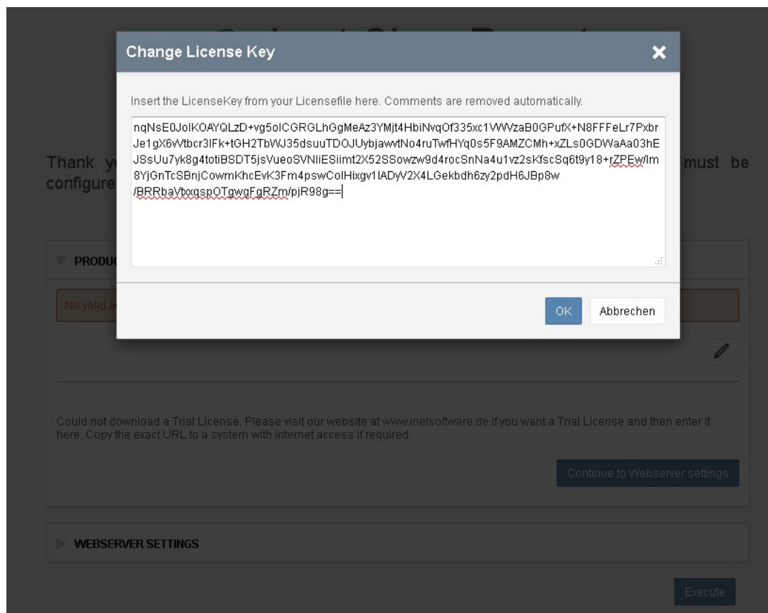
Figure 10-30 Entering the i-net Clear Reports 17.x License
