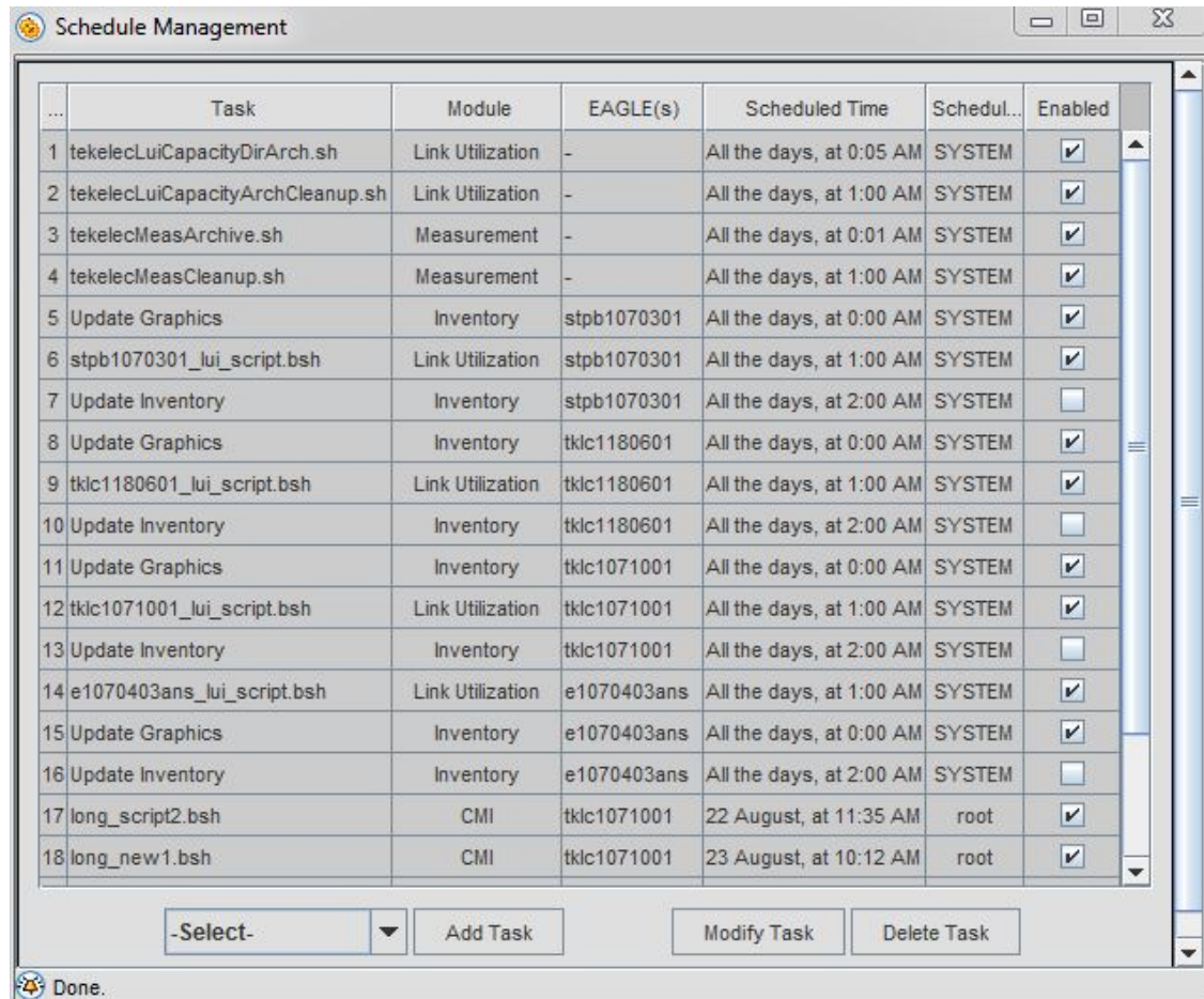
Figure 5-18 Schedule Management Screen
