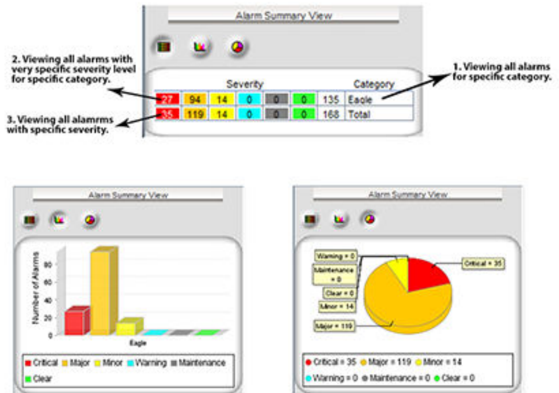
Figure 4-10 Alarm Summary Views
