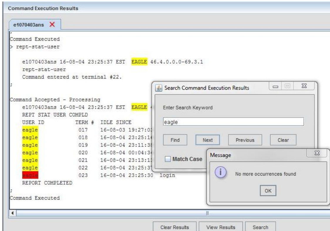
Figure 11-12 Send Command Search
