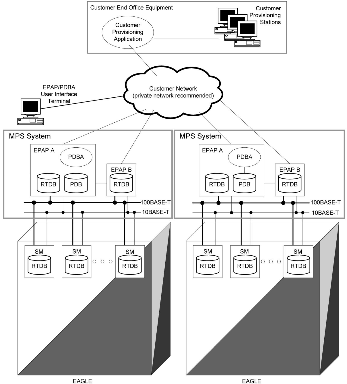
Figure 2-1 Generic EPAP Deployment Model
