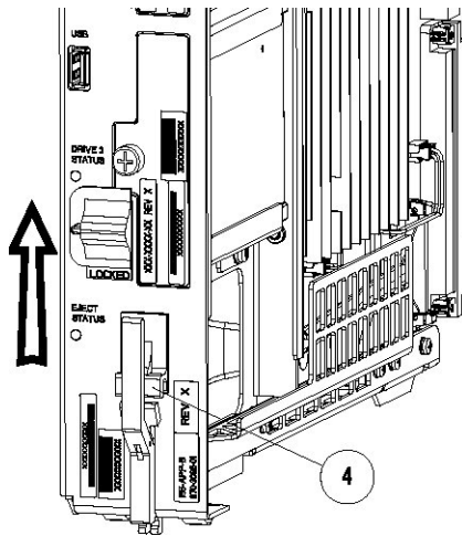
Figure 5-1 E5-APP-B Card Eject Hardware Switch, UNLOCKED
