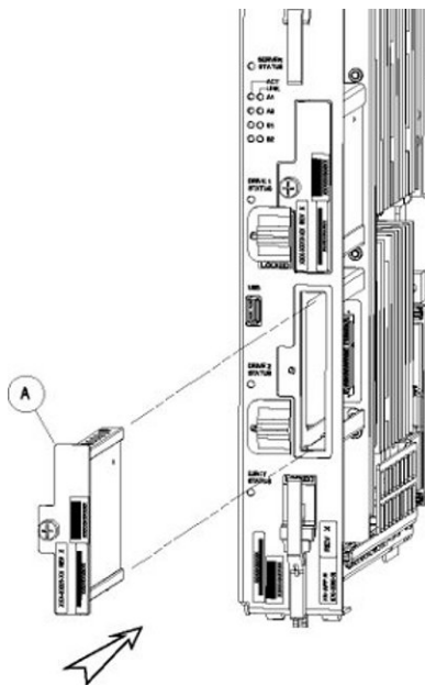
Figure 5-10 Drive Module Replacement
