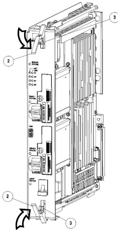
Figure 5-4 E5-APP-B Card Inject Levers
