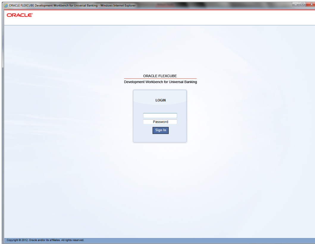
Fig 3.1: Login Screen
