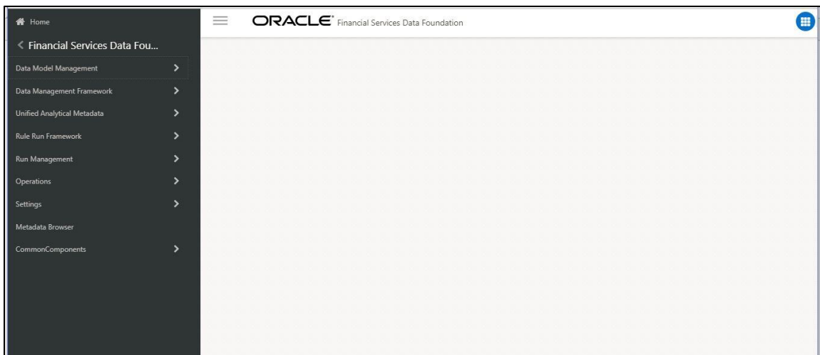
Figure 4: Home Page
