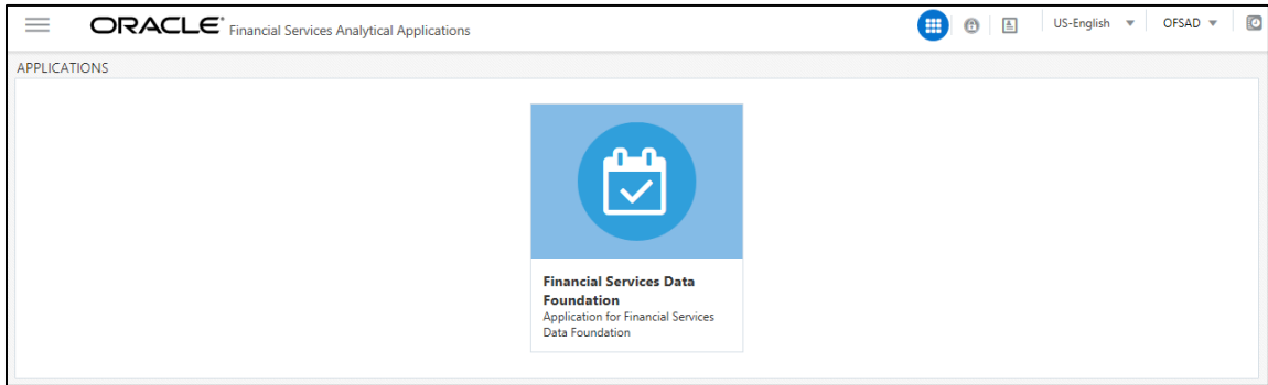
Figure 3: Landing Page
