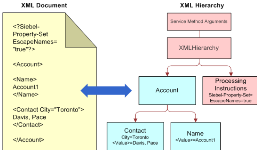
Figure 6. XML Hierarchy Representation of XML Document Structure
