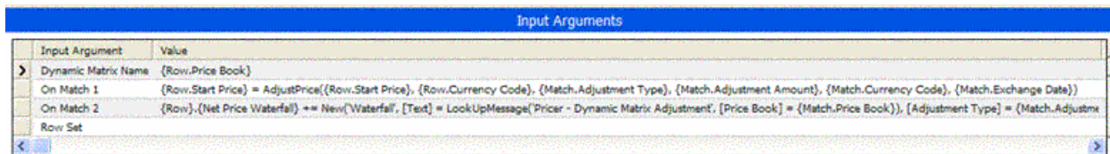
Figure 23. Example of Arguments for Dynamic Look-Up Method
