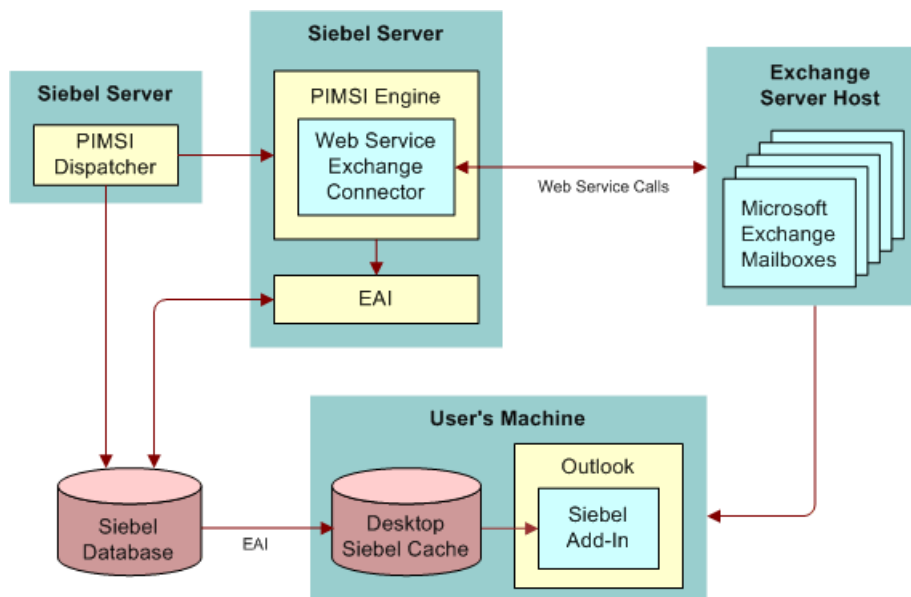
Figure 3. SSSE Architecture
