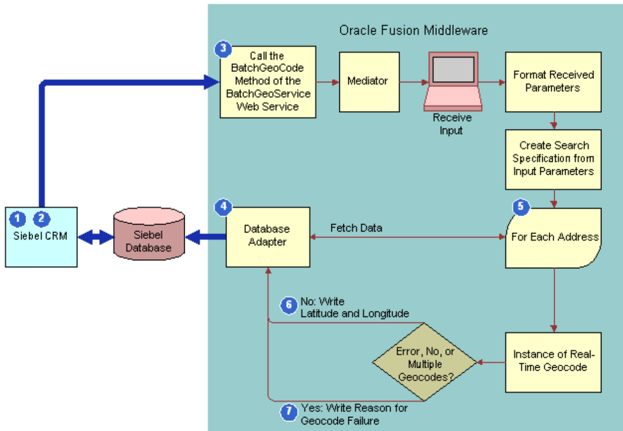
Figure 13. Integration Flow That Retrieves Geocodes for Multiple Addresses
