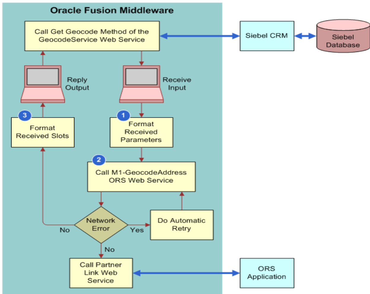
Figure 12. Integration Flow That Retrieves a Geocode for a Single Address in Real-Time
