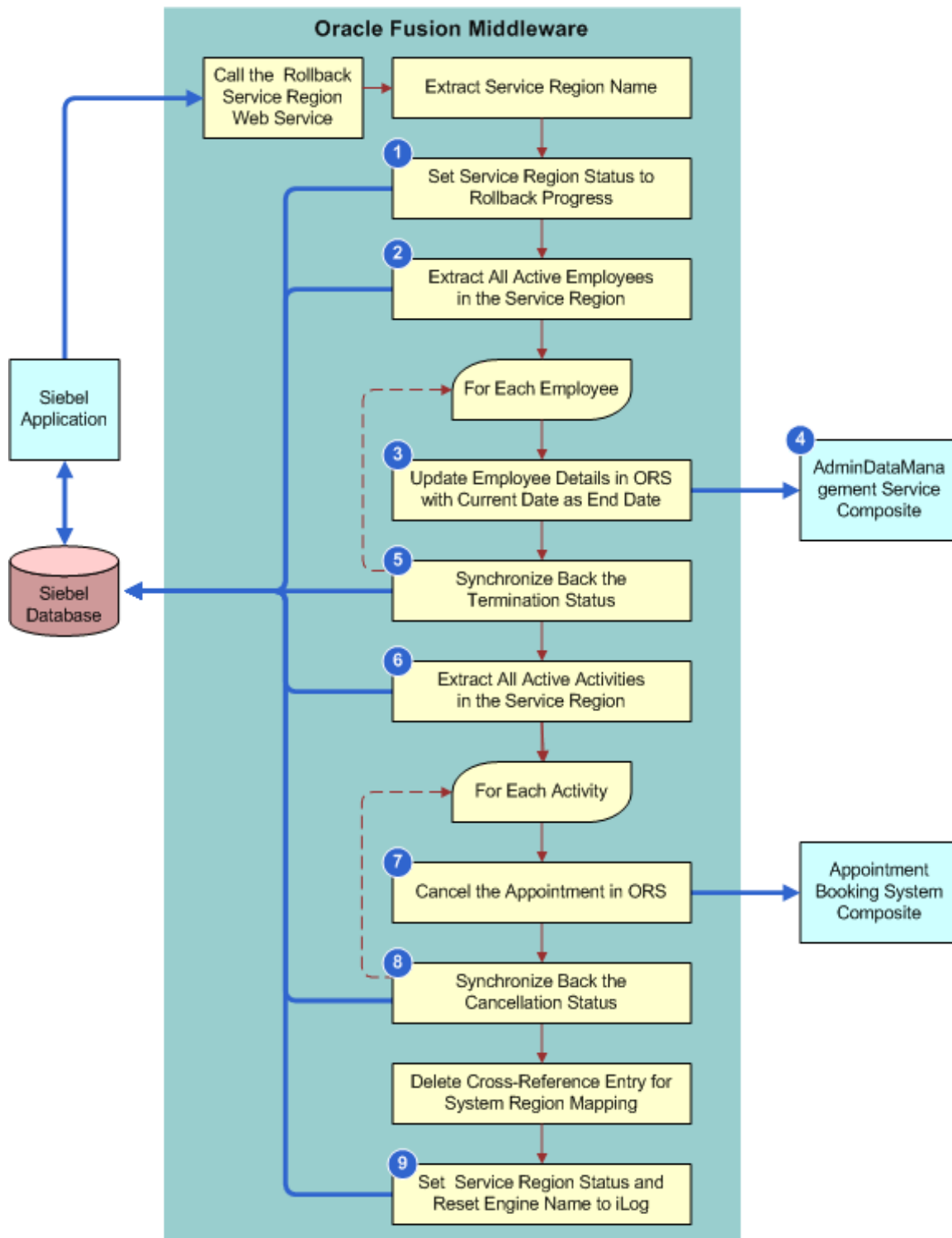
Figure 15. Integration Flow to Perform a Service Region Rollback
