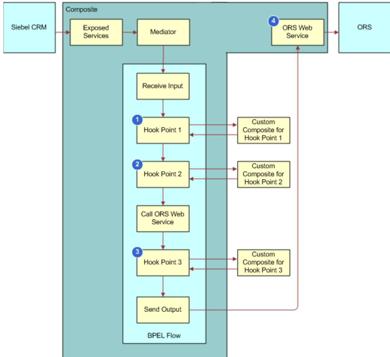
Figure 16. Generic Flow That Includes Hook Points
