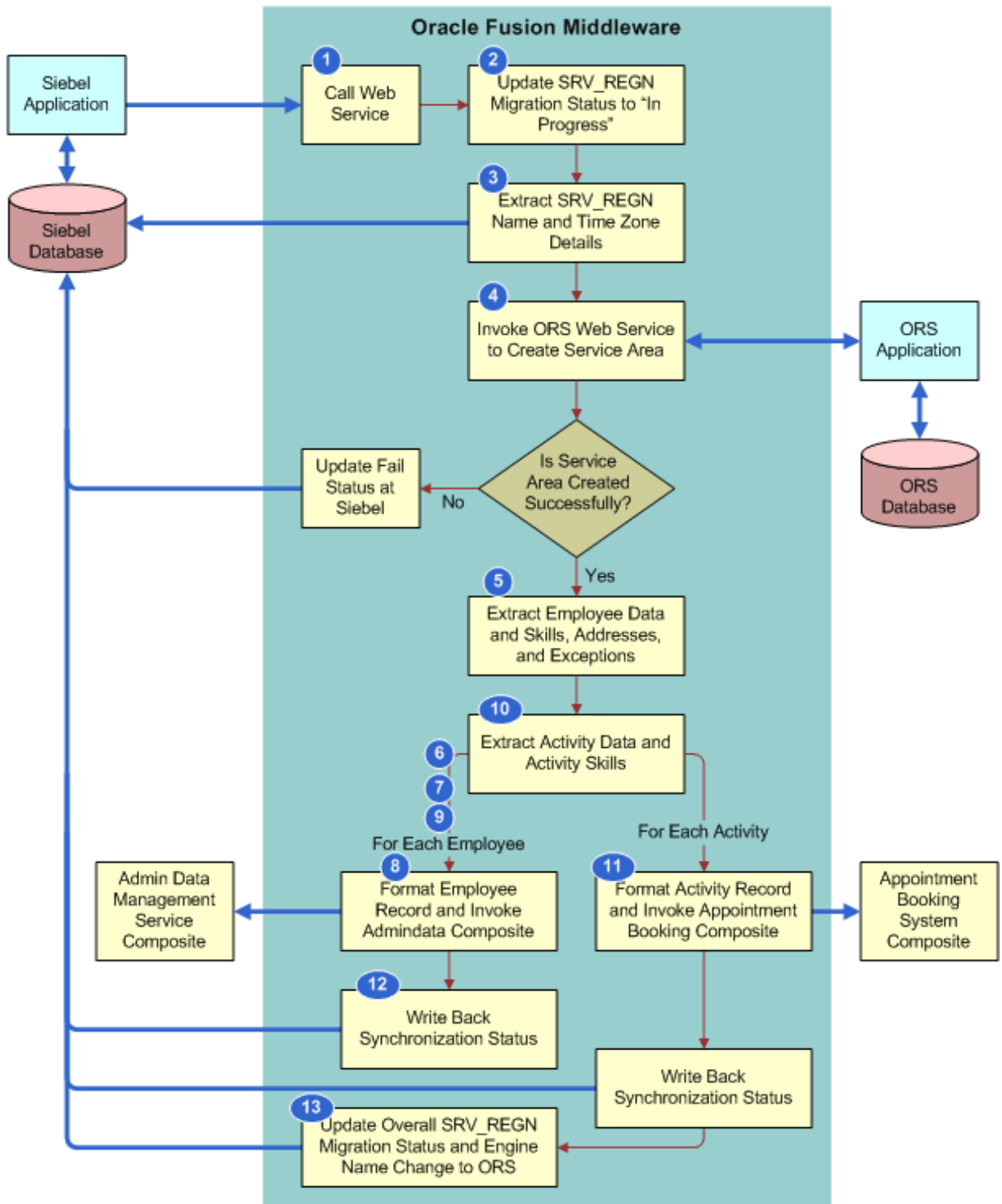
Figure 14. Integration Flow to Perform a Service Region Data Transfer
