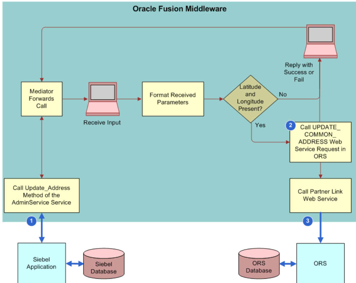
Figure 11. Integration Flow to Update or Insert an Address
