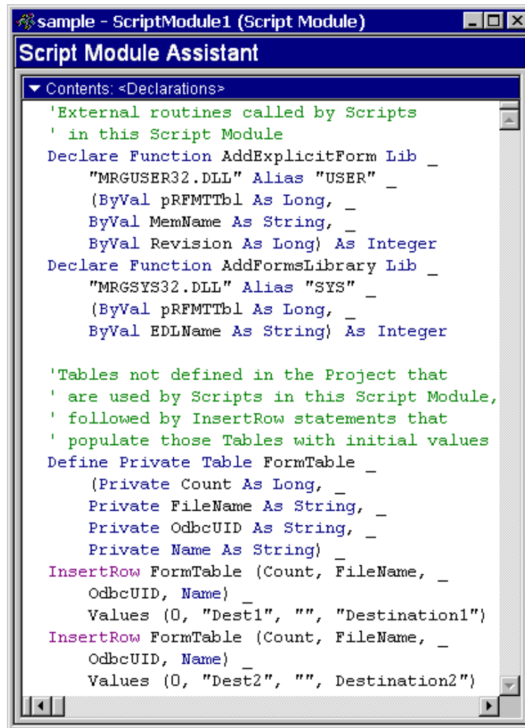
Figure 2: Declarations Section That Declares External Routines and Noncomponent Table
