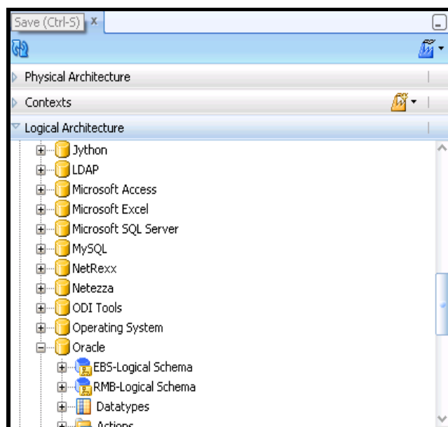
Figure 15: Logical Architecture
