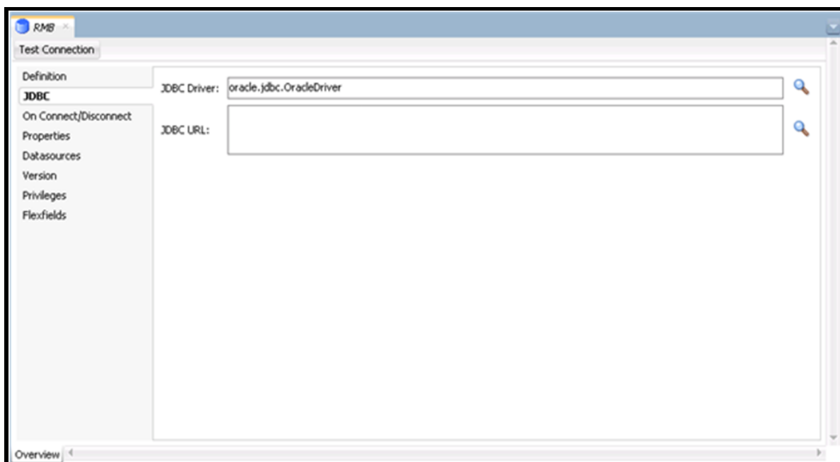
Figure 12: JDBC Tab
