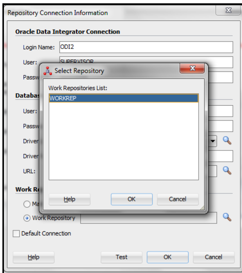
Figure 7: Select Repository
