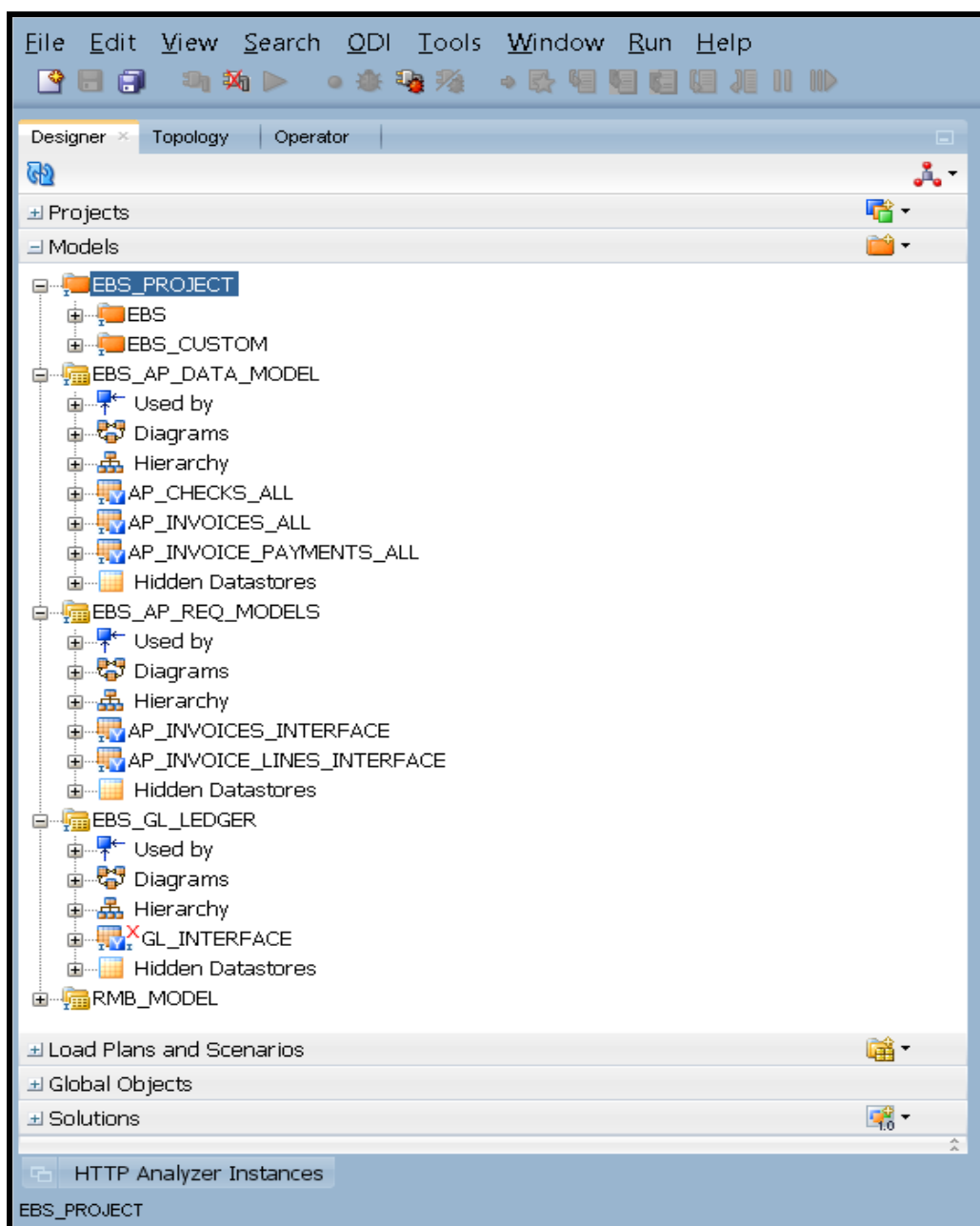
Figure 9: Designer Tab
