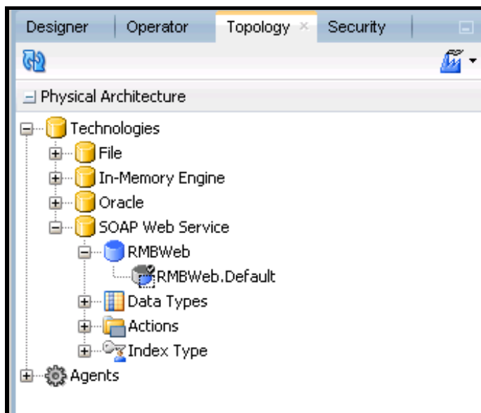
Figure 16: Physical Architecture
