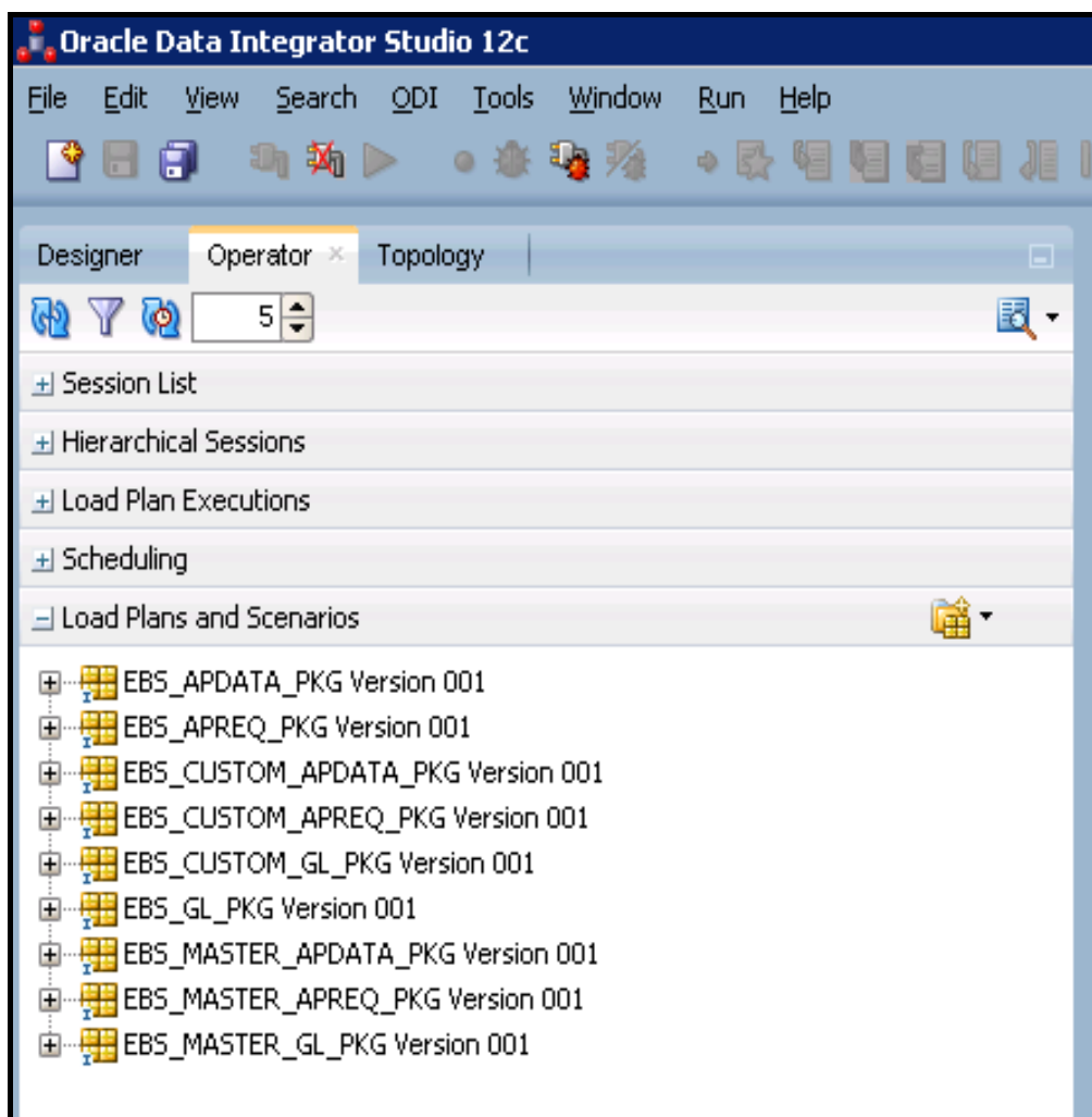
Figure 10: Operator Tab
