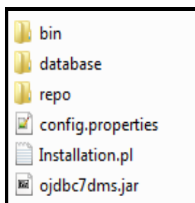
Figure 1: Directory Names
