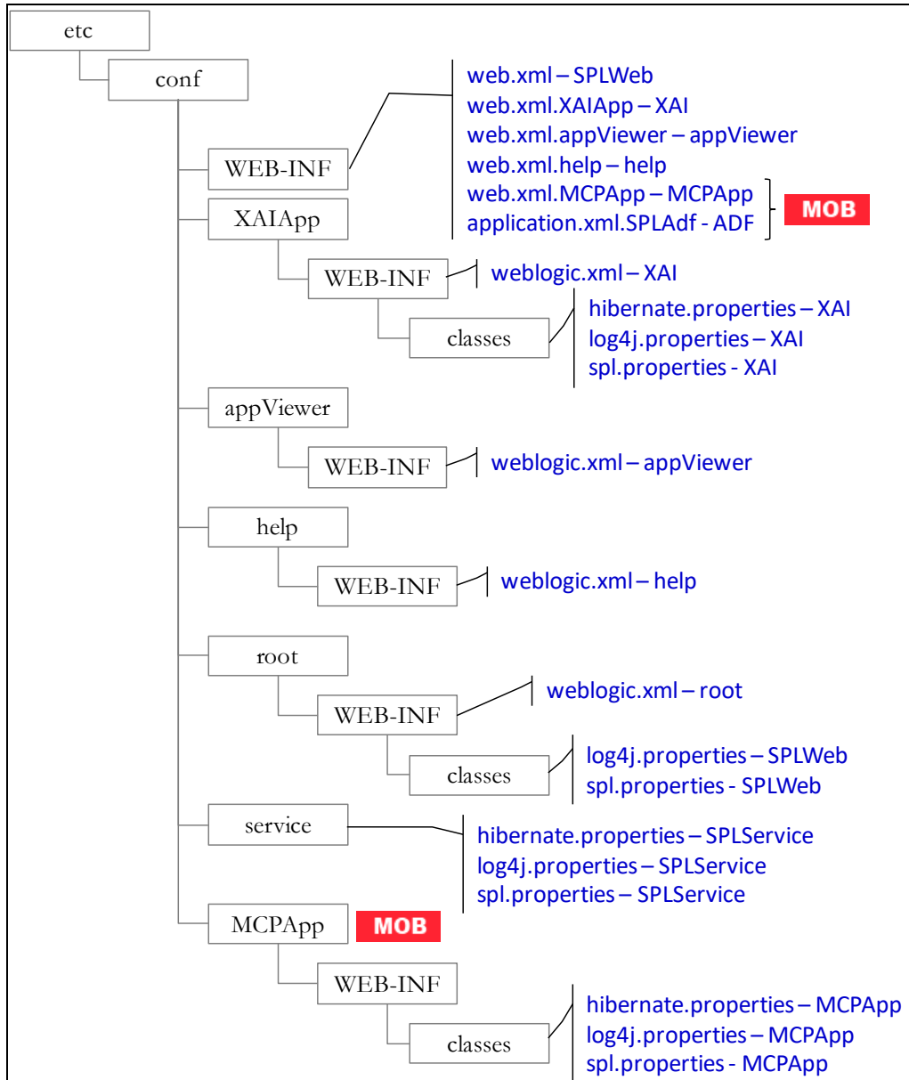
Figure 22: Configuration File Hierarchy
