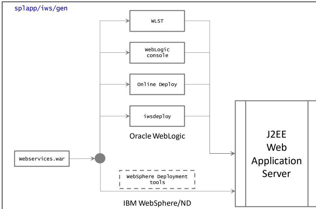
Figure 32: Inbound Web Services Deployment Process
