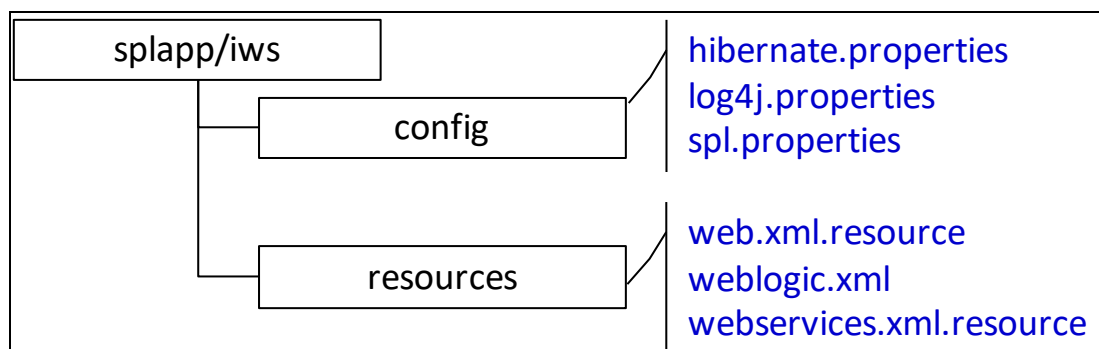
Figure 29: Inbound Web Services Configuration
