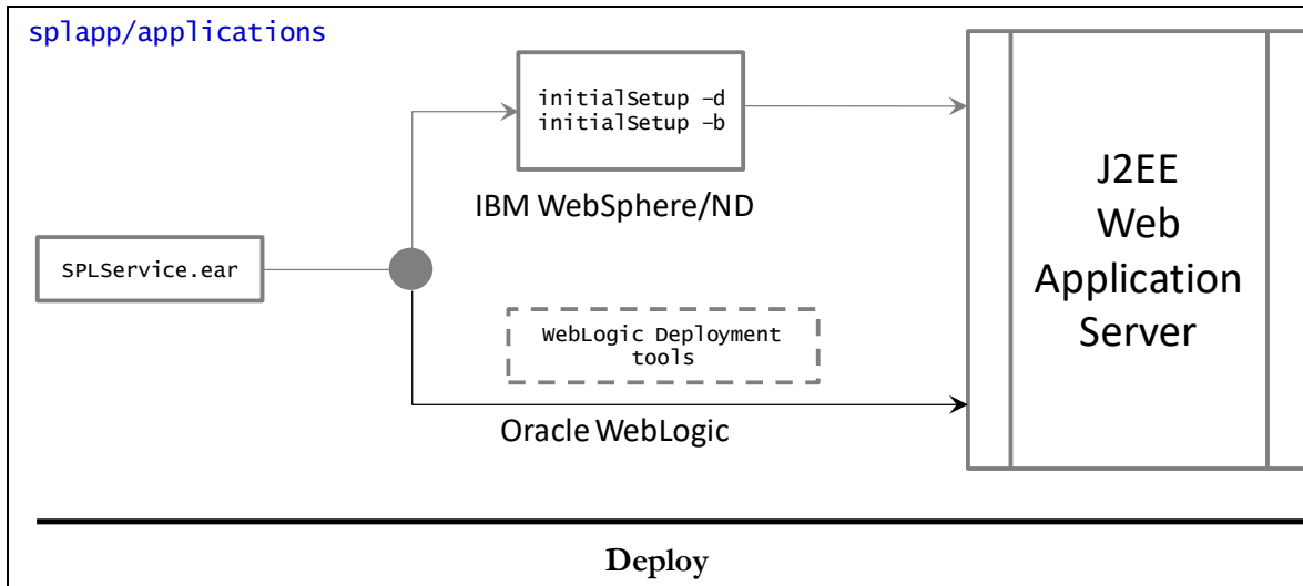
Figure 28: Business Application Server Deployment Process
