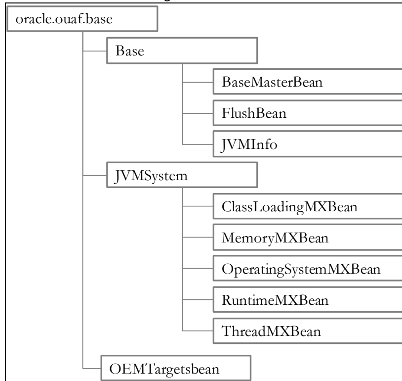
Figure 13: Web Application Server Mbeans
