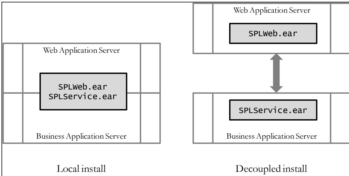
Figure 25: Installation Modes
