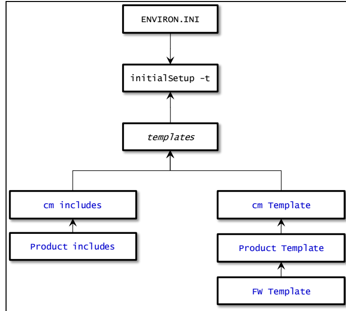
Figure 41: Template Hierarchy
