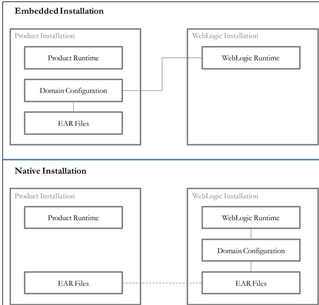
Figure 4: Native and Embedded Architectures
