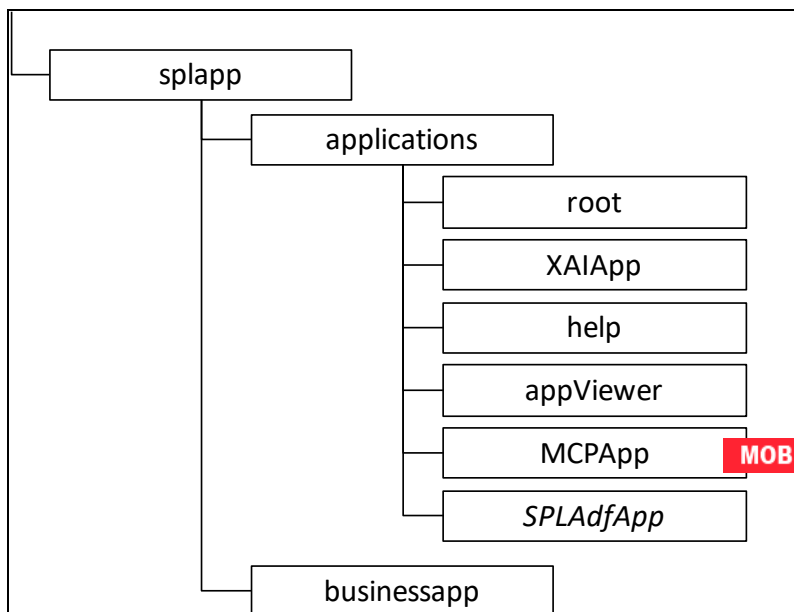
Figure 39: Expanded Format
