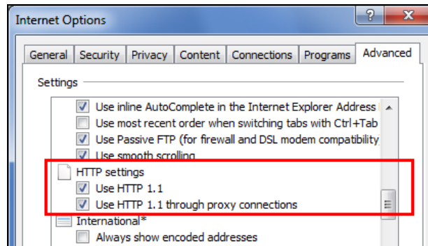
Figure 19: HTTP 1.1 Settings
