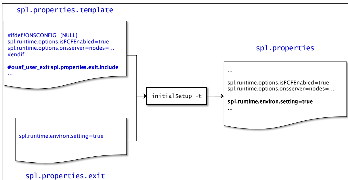
Figure 40: Include Files
