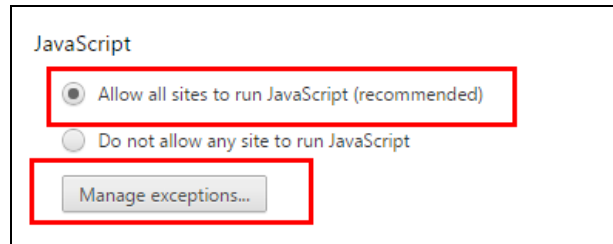
Figure 20: Javascript Settings
