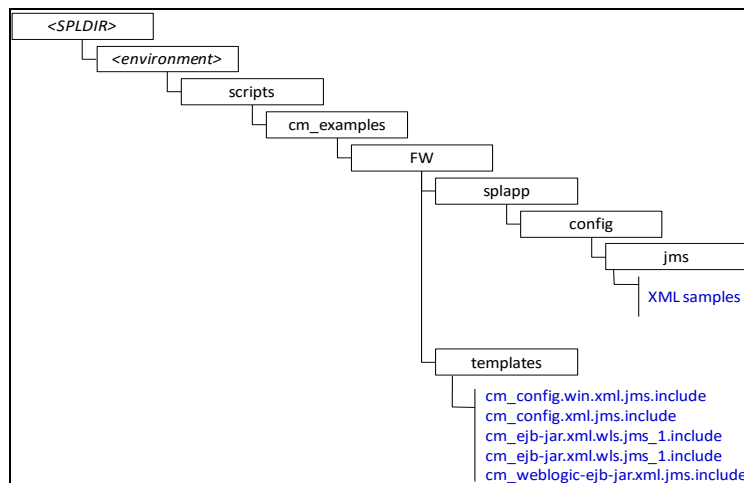
Figure 42: Custom JMS Configuration
