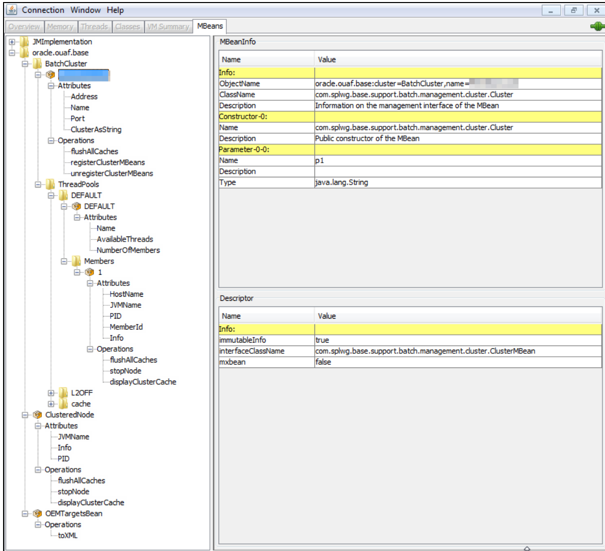
Figure 16: Batch Server Mbeans in jconsole Example
