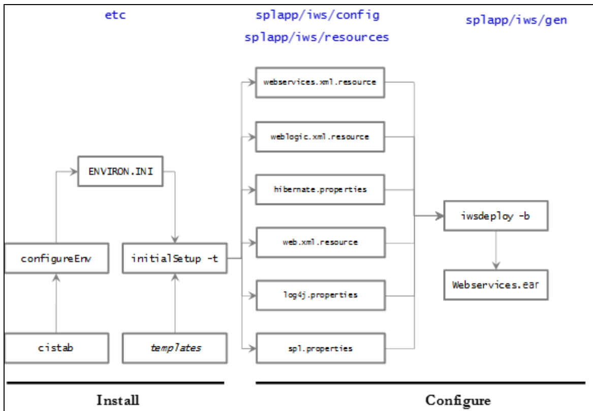
Figure 31: Inbound Web Services Configuration Process
