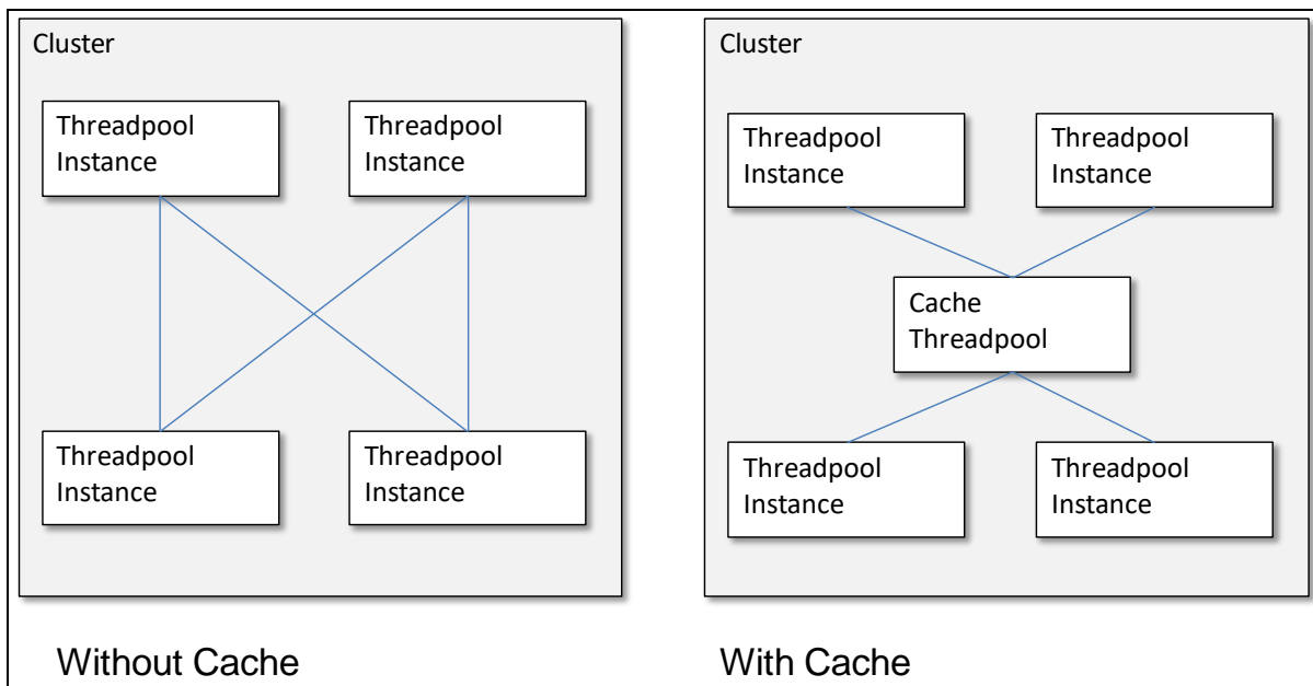
Figure 37: Cache Architecture
