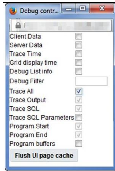
Figure 11: Debug Controls
