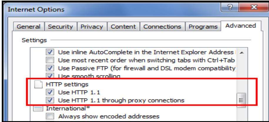
Figure 19: HTTP 1.1 Settings
