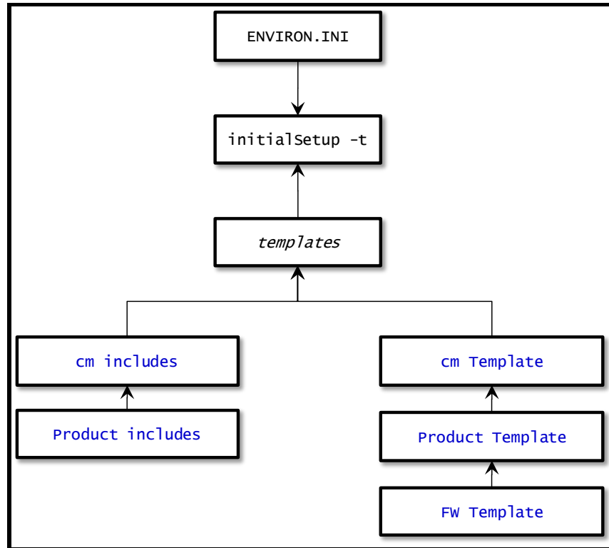
Figure 41: Template Hierarchy
