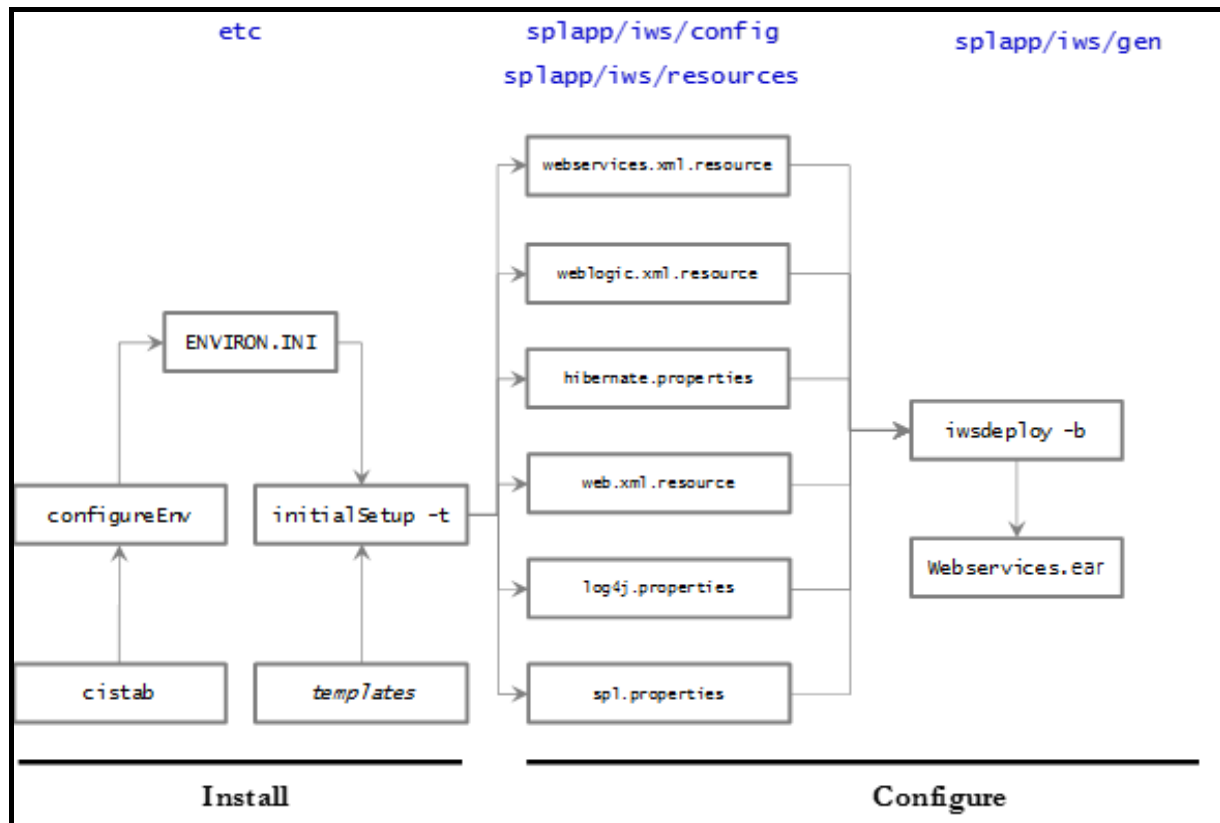
Figure 31: Inbound Web Services Configuration Process
