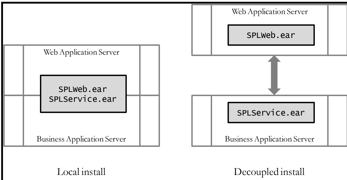
Figure 25: Installation Modes
