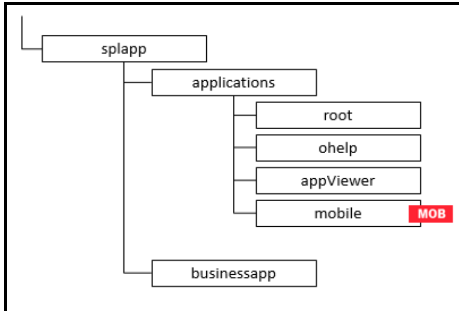
Figure 39: Expanded Format
