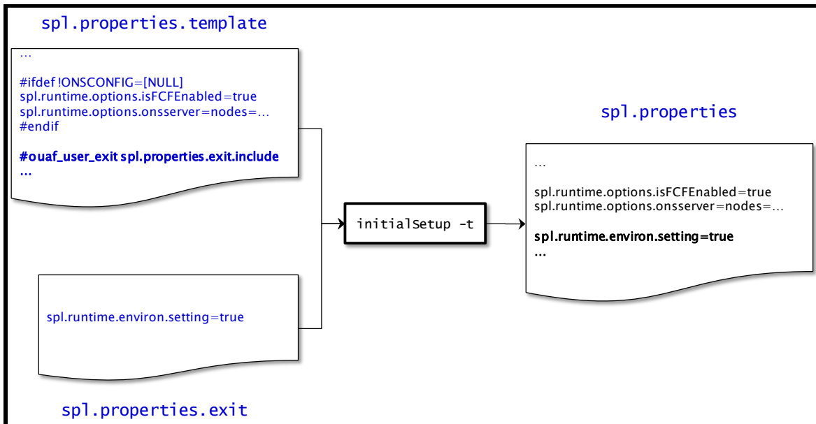
Figure 40: Include Files
