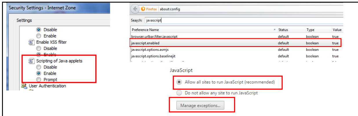
Figure 20: Javascript Settings
