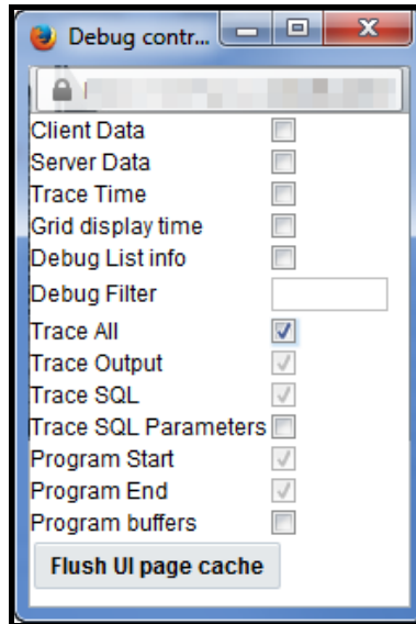
Figure 11: Debug Controls
