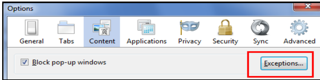
Figure 21: Exceptions
