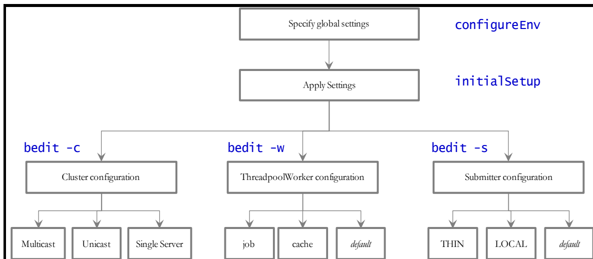
Figure 36: bedit Configuration Process
