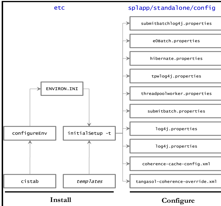
Figure 35: Batch Configuration Process
