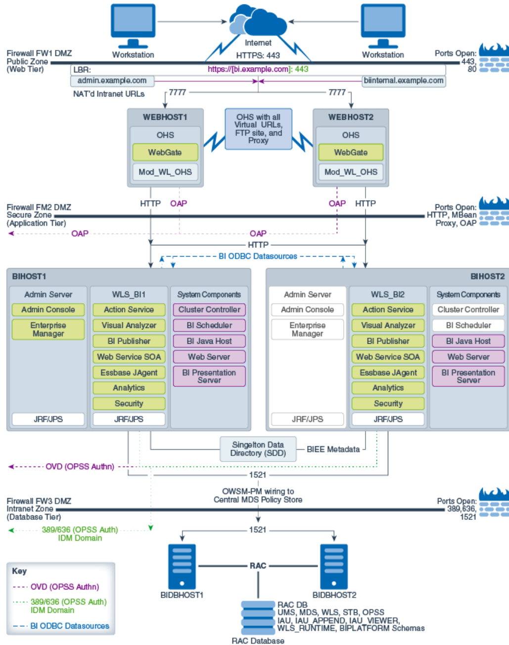
Figure 3-1 Primary Business Intelligence Enterprise Topology
