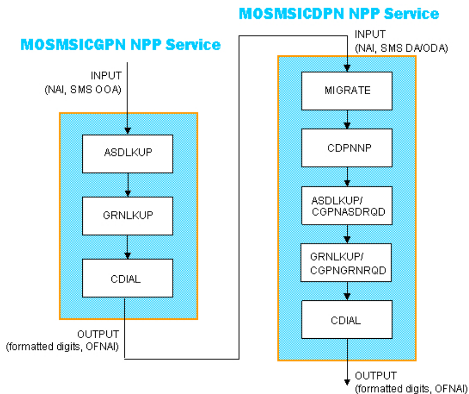
Figure 2-10 MO SMS NPP - IS41 Processing
