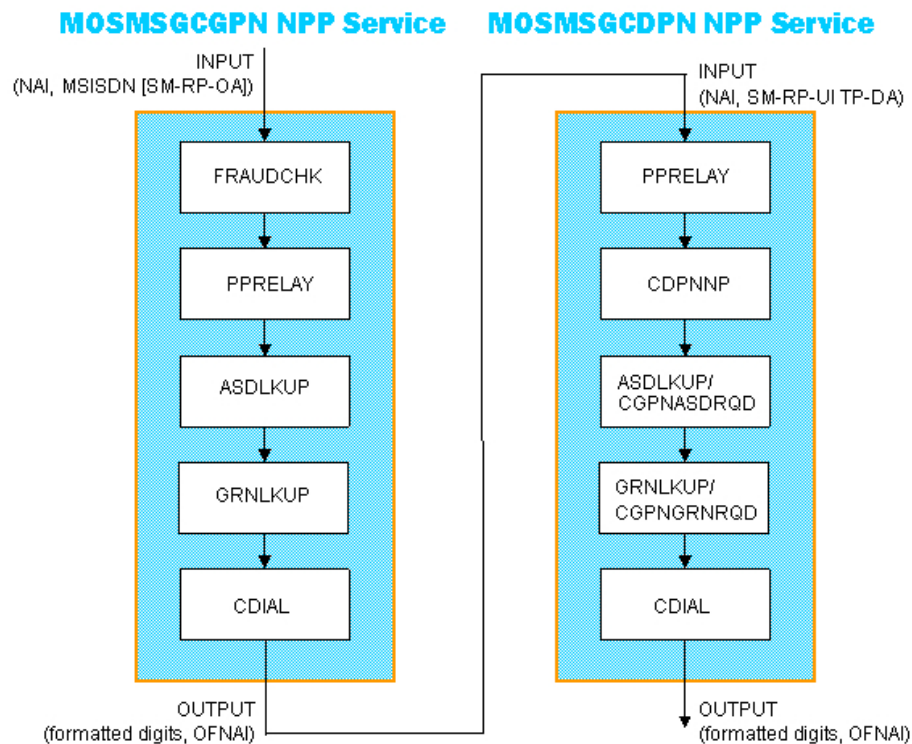
Figure 2-9 MO SMS NPP - GSM NPP Processing
