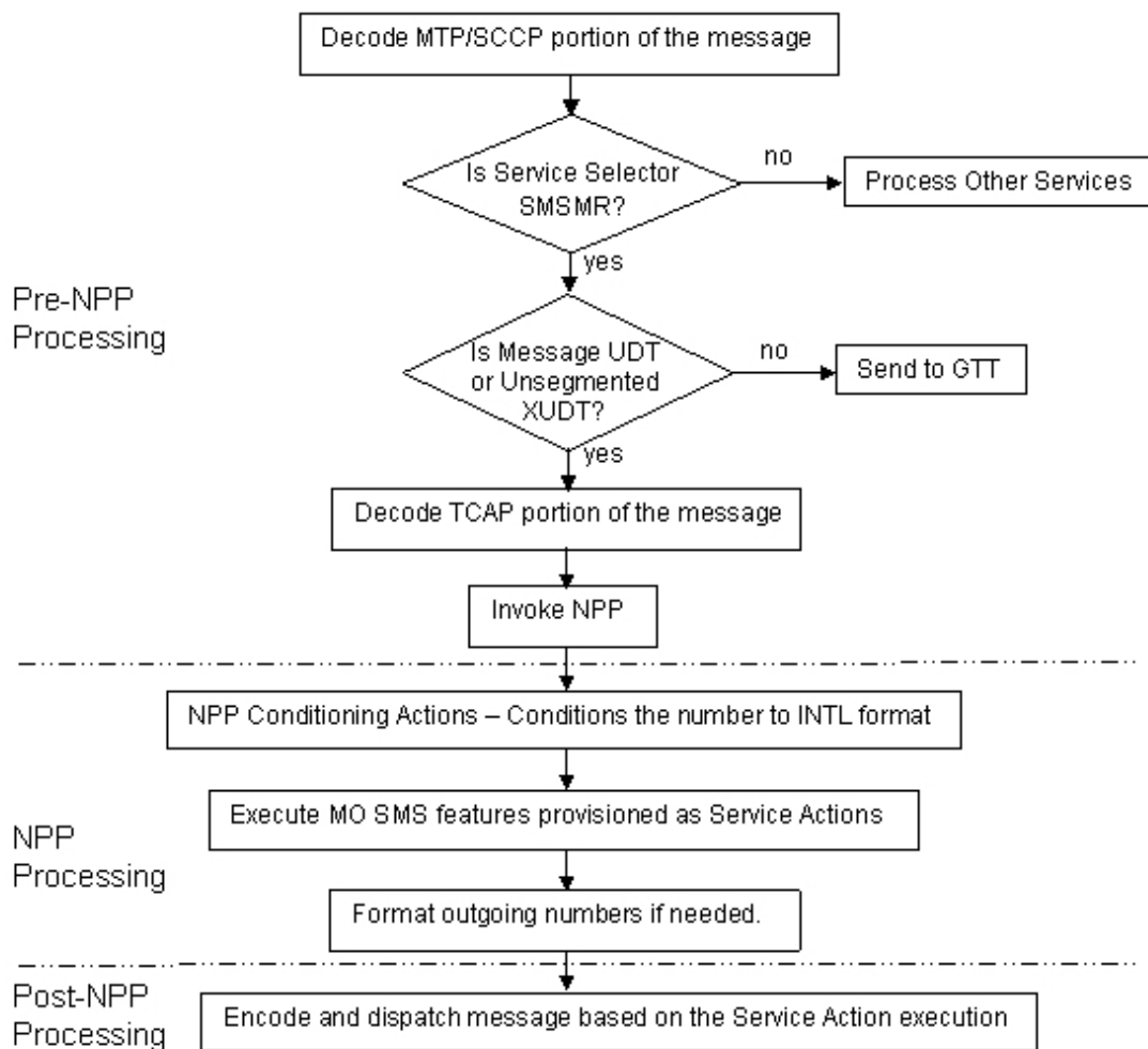
Figure 2-8 MO SMS NPP Message Processing
