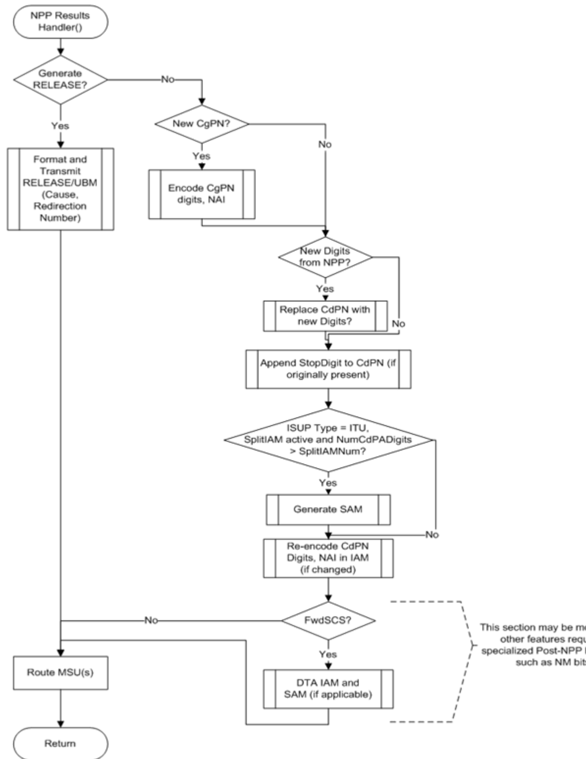
Figure 2-6 TIF Post-NPP Results Handler
