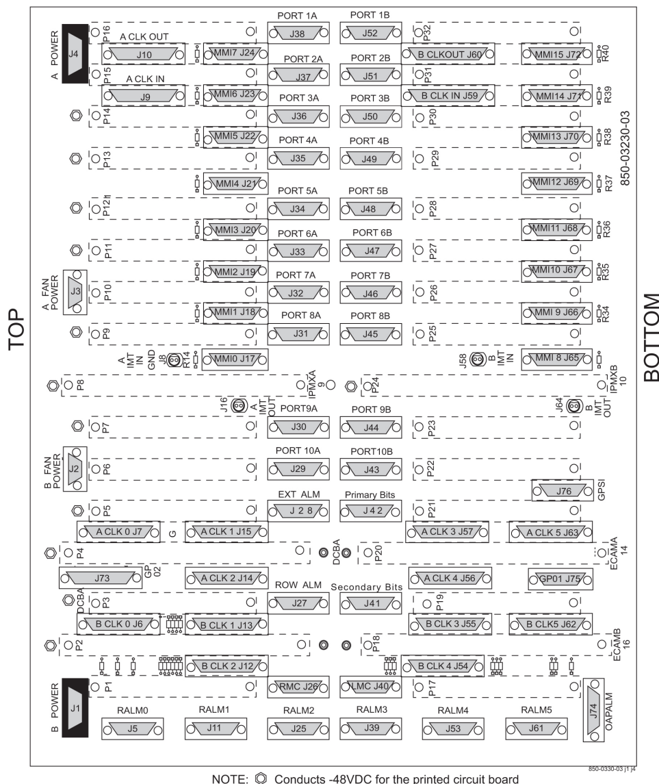
Figure 3-16 Control Shelf Backplane (P/N 850-0330-03/04)
