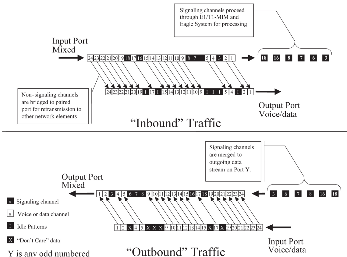
Figure 3-37 Channel Bridging Schematic
