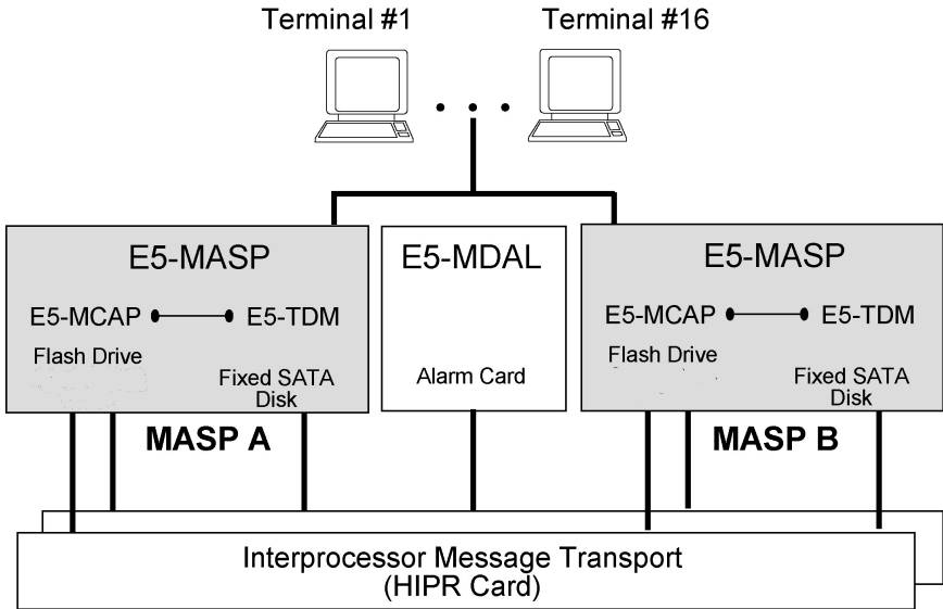
Figure 2-2 E5-based Maintenance and Administration Subsystem Block Diagram
