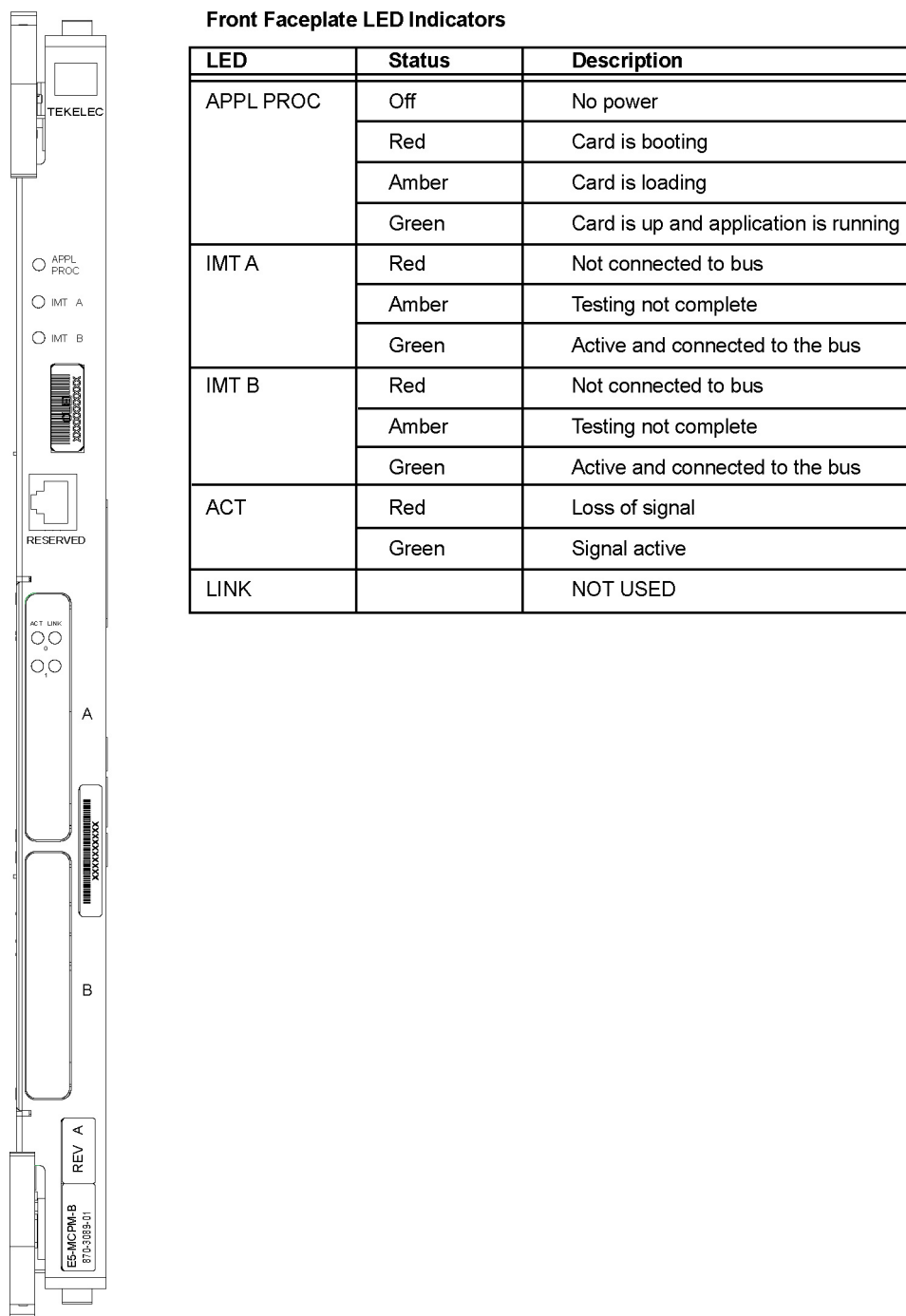
Figure 3-41 E5-MCPM-B
