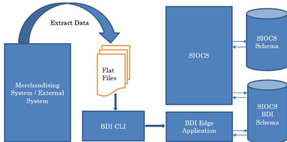
Figure L-1 Transaction Import Process Flow
