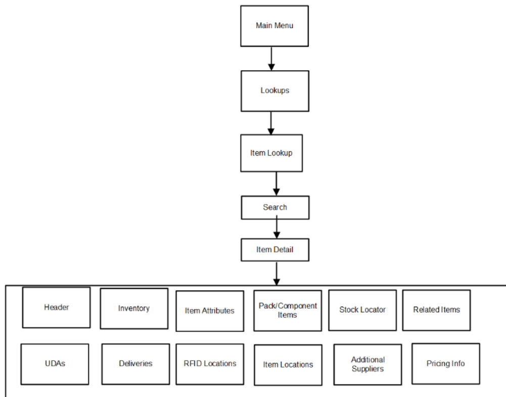
Figure 10-1 Item Lookup Screen Flow
