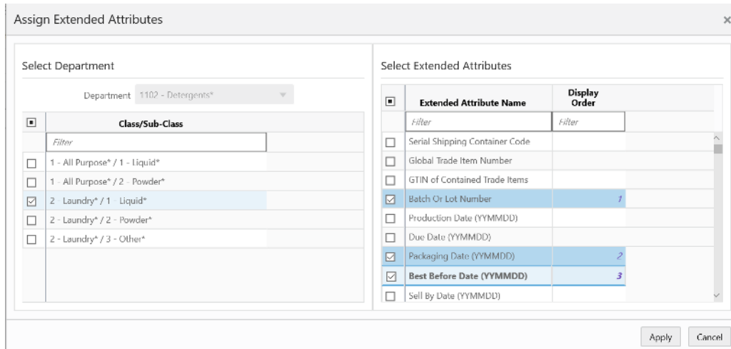
Figure 3–15 Assign Extended Attributes Popup
