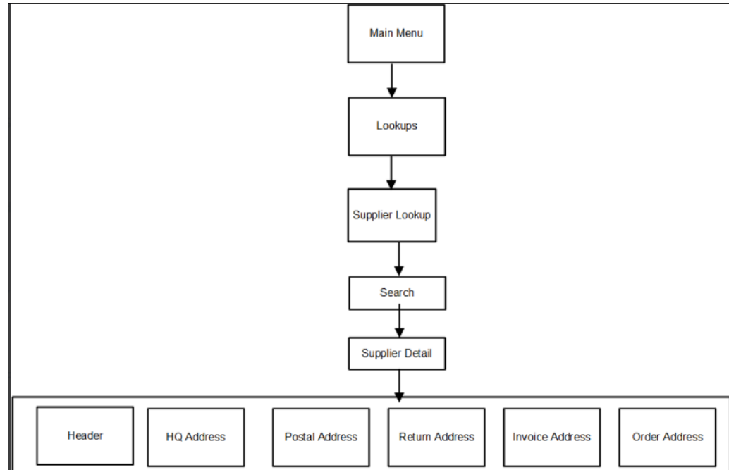
Figure 10–27 Supplier Lookup Workflow
