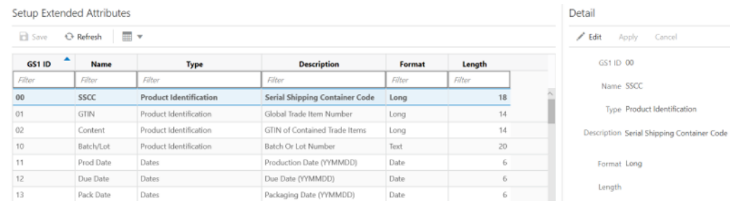
Figure 3–13 Setup Extended Attributes Screen
